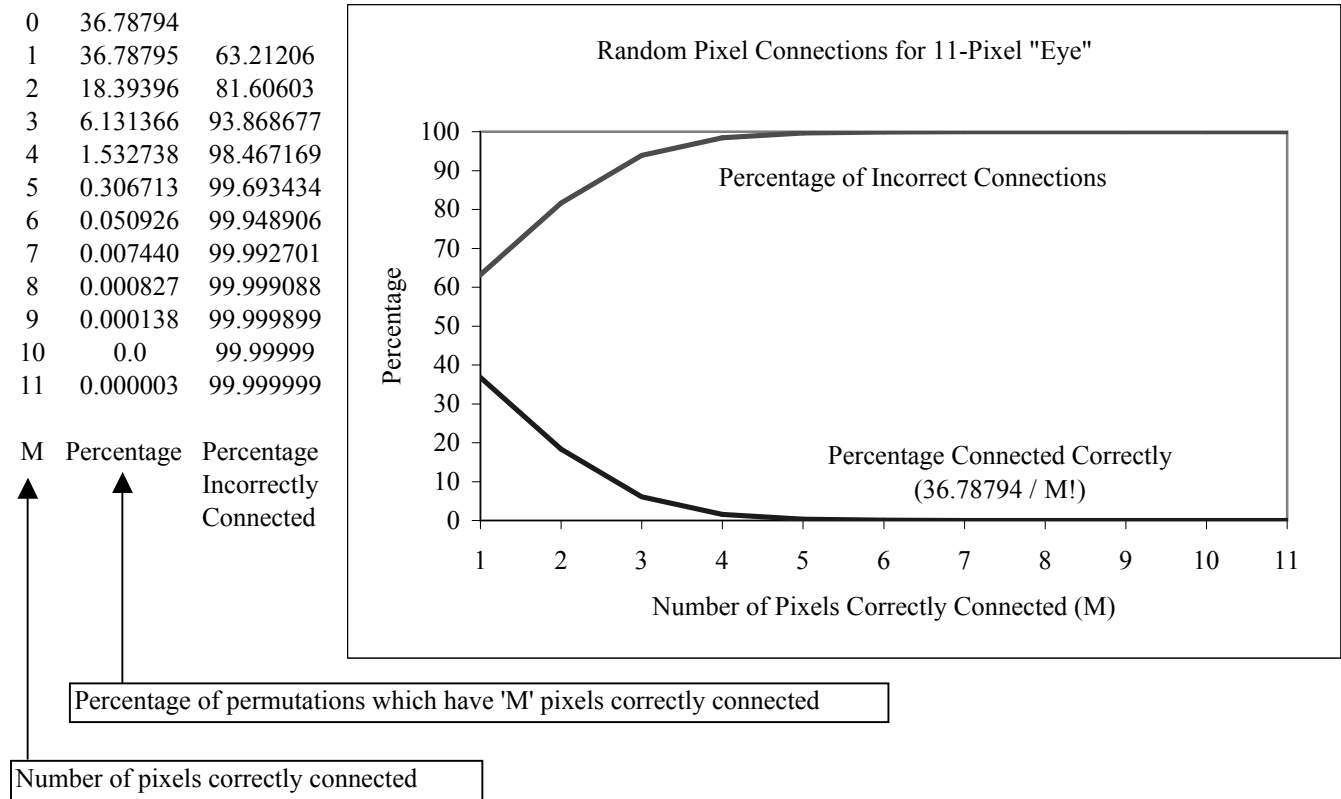
Figure 7. Statistics for randomly connecting an 11-pixel eye.
