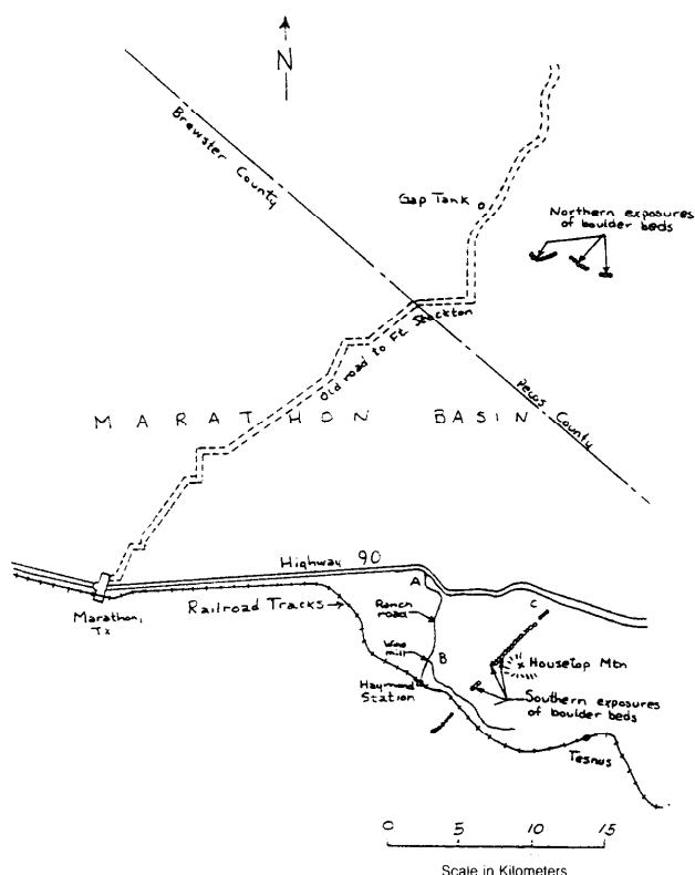
Figure 1. Map showing southern and northern exposures of the boulder beds in the Haymond Formation. Map redrawn from Hall (1957, p. 1634) by Brenda L. Lindley-Anderson.
