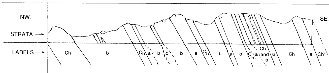
Figure 11. A diagrammatic cross section of the boulder bed member of The Haymond Formation at one location in its southern exposure; after King (1937, p. 67). Labels are as follows: Ch, thinbedded sandstone and shale (flysch); Ch', a more shaly phase; a, arkose beds; b, boulder-bearing mudstone; c, breccia. King's original section shows some of the larger "Pennsylvanian limestone," Caballos novaculite, and Dimple limestone in place. No attempt has been made to include those individual boulders here as King did in the original but they all occur in beds labeled b—boulder-bearing mudstones. Alluvium and gravel deposits present at certain localities on the original are not shown here. It is readily obvious in this figure that the boulder-bearing mudstones alternate with beds of arkose and with the sandstone-shale interbed strata.
