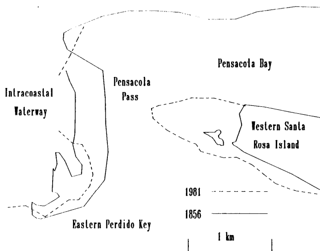
Figure 1. Shoreline changes near Pensacola, Florida. Based on a figure from Stone (1984), reprinted in Coleman (1988).
