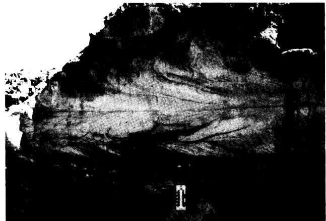
Figure 4. This is a closeup photograph of a cliff sidewall seen in Figure 1, showing semi-consolidated crossbedded sands which have contributed to the rapid development of the small-scale canyon. Scale is in inches and centimeters.
