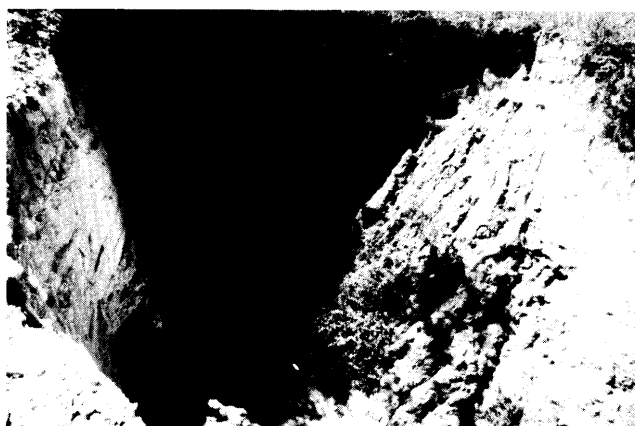
Figure 1. Cliff sapping of sidewalls. Note soil mass slumped at the base of the cliff face. This canyon was initiated with the construction of a nearby drainage ditch. The depth from the ground surface to the base of the pit, in this photograph, is approximately 18 feet. No surface stream is associated with this feature. Benton County, MS.
