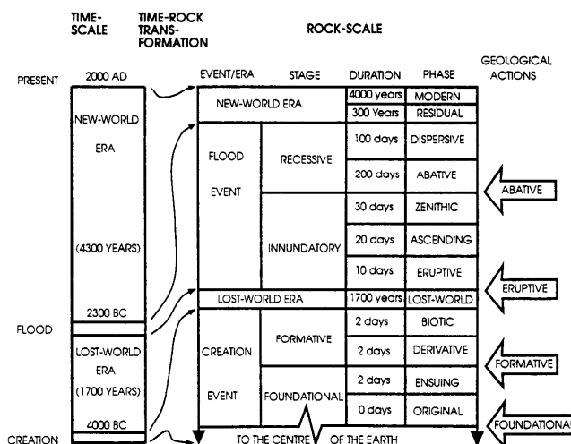
Figure 1. The Pittsburgh Biblical geological model (After Walker, 1994).
