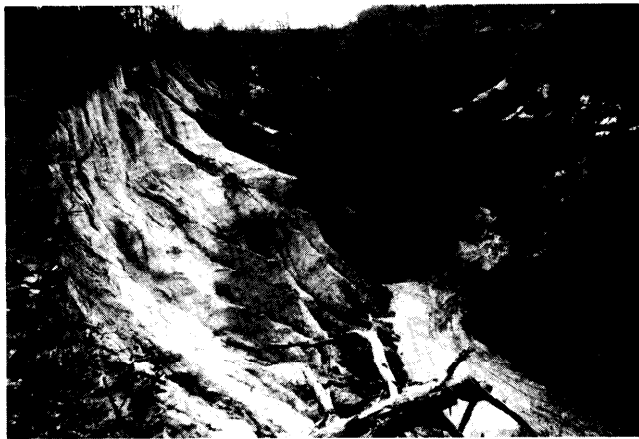
Figure 3. Unnamed Canyon located approximately one mile northeast of Providence Canyon, Stewart County, Georgia, along Georgia Highway 39c. This canyon exhibits badlands topography which is a geomorphic surface expression which the nearby Providence Canyon are also noted. The depth from the ground surface to the base of the pit, in this photograph, is approximately 199 feet. No surface stream is associated with this feature.
