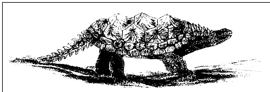
Figure 2. Artist Lisa Pizzarella's conception of Proganochelys quenstedtii . Drawing supplied through the courtesy of Dr. Wayne Frair.
