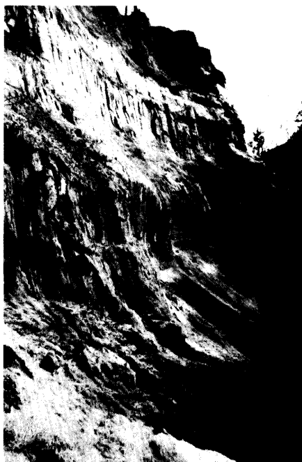
Figure 6. This photograph shows a multi-tiered sidewall exposed in one of the canyons at Providence Canyon. The reason for the tiering is due to stratification of the individual layers. Some layers weather more rapidly than others and this creates the stair-step nature of the canyon sidewalls. This sidewall is 75 feet high in this photograph.
