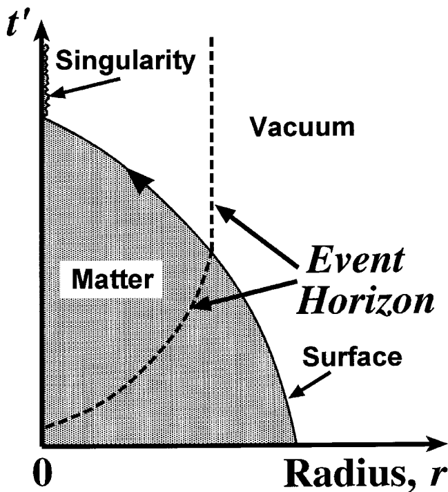
Figure 1. A collapsing ball of matter can contain an event horizon. Figure adapted from Figure 57 (i) of Hawking and Ellis (1973, p. 309). The horizontal axis is the Schwarzschild radial distance, r , from the center of the ball. The vertical axis is a time coordinate, t' . (Specifically, it is the Eddington-Finkelstein time coordinate, the sum of the Schwarzschild time t plus a function of r .) The shaded part of the figure represents the interior of the ball. The dotted line shows the event horizon, where time dilation occurs.
