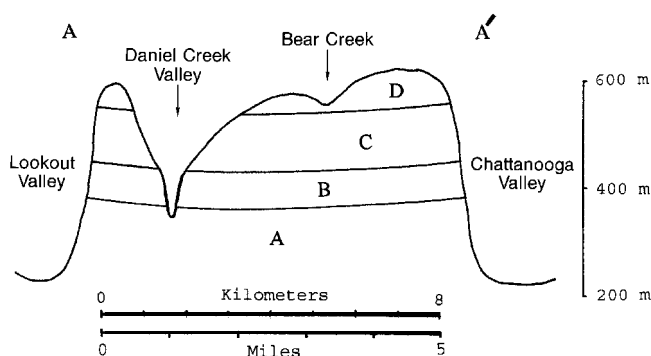
Figure 5. Northwest (A) to southeast (A') generalized cross-section across the Lookout Mountain Ridge. The line of section is shown in Figure 1a. The slight upward curve of the strata reflect the synclinal shape of the ridge. Note that the scale is exaggerated. The vertical scale is based on relative sea-level. The top surface of the Lookout Mountain Ridge dips toward the northwest and serves to direct the overland flow of water towards Lookout Valley. This overland flow from Lookout Mountain Ridge has resulted in the formation of Daniel and Bear creeks and their respective canyons. Generalized stratigraphic section is presented as: A) Pennington Formation (Mississippian), B) Raccoon Mountain Member, C) Warren Point Member, and D) Sewanee Member-all part of the Gizzard Formation (Pennsylvanian).
