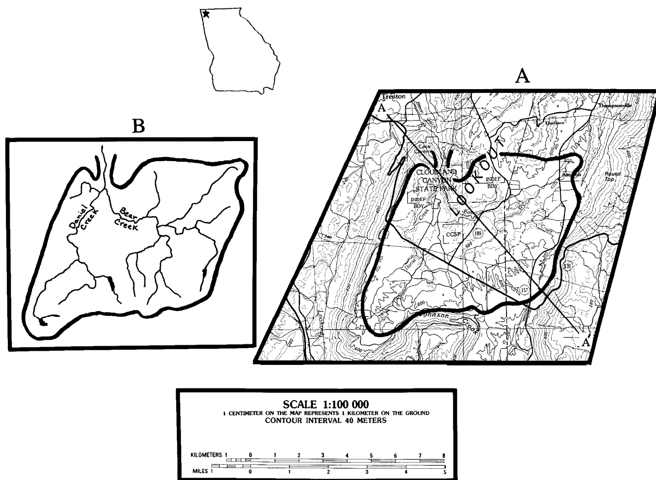
Figure 1. a) U.S. Geological Survey map showing the general area surrounding Cloudland Canyon State Park. Generalized cross-section is represented in diagonal line (see Figure 5). Note sizes of the canyons which are said to represent 300 million years of erosion. b) A watershed map at the same scale as the topographic map. This map shows the areas drained by both Daniel Creek and Bear Creek. The amount of time of erosion postulated for this site (i.e., 300 million years) should result in a larger watershed than is found. Additionally, canyon development should be much more extensive. The millions of years of "ice age" precipitation (uniformitarian estimate) alone should have resulted in greater canyon development than what is found at present. Note the size of the areas drained.
