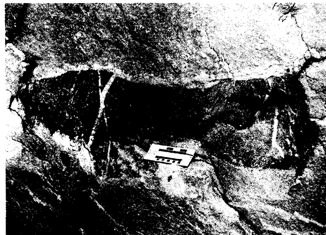
Figure 2. Xenolith exposed in the former granite quarry located on the east end of the Stone Mountain pluton. This area has undergone extensive granite removal and it can be estimated that several feet of overlying granite have been removed to expose this biotite gneiss xenolith. Note the somewhat rounded contact surface with the surrounding Stone Mountain Granite. Scale in inches and centimeters.
