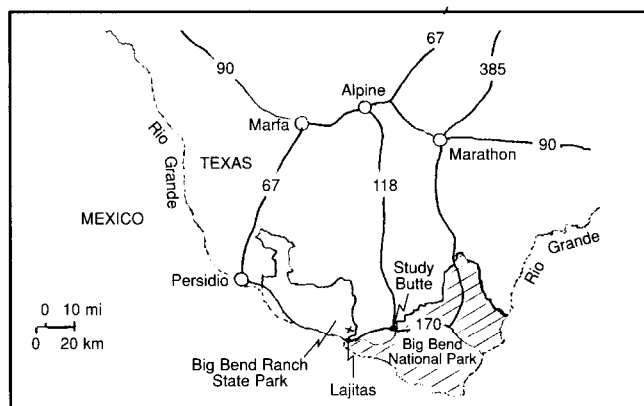
Figure 2. Location (x) of amphitheater in Terlingua monocline north of Lajitas, Texas within Big Bend Ranch State Park in relation to the major highways (numbered) and towns in this region of Trans-Pecos Texas.
