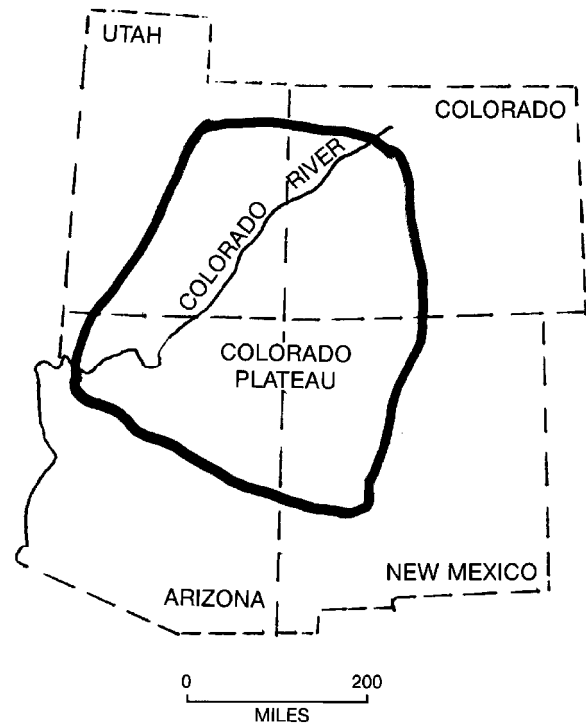
Figure 3. Location of the Colorado Plateau in the western United States (after Huntton, 1989, p. 73).
