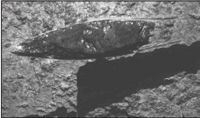
Figure 1. Mid-sized nautiloid fossil, Hook Island, Ontario. Length approximately 50 cm.
