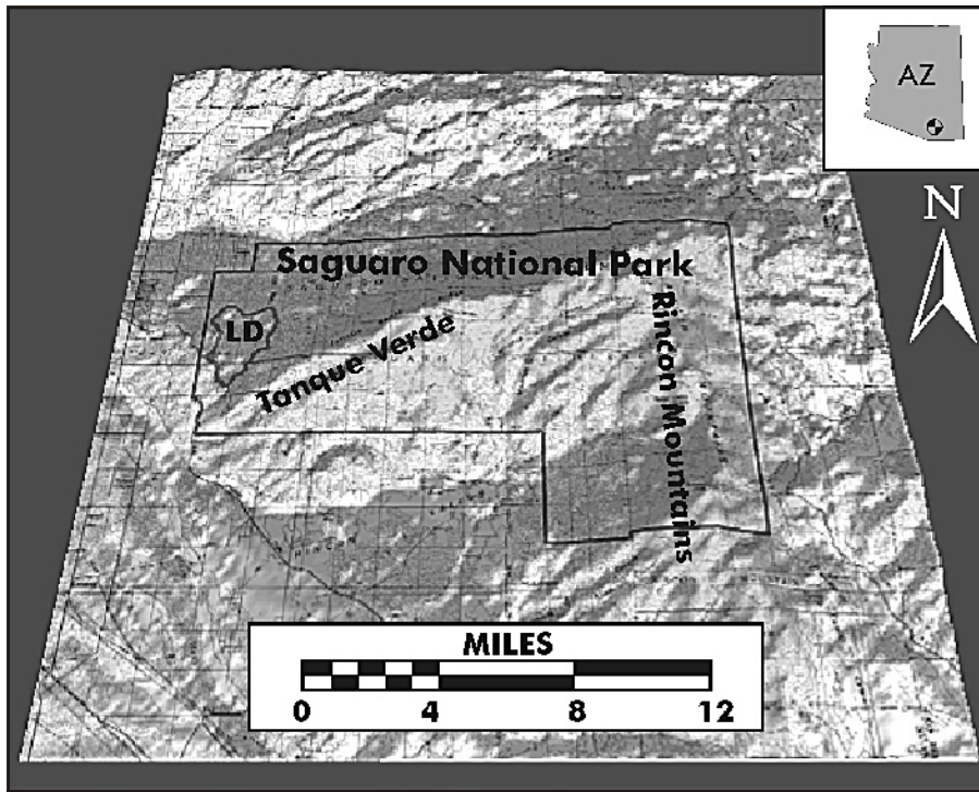
Figure 1. Topographic map showing the extent of Saguaro National Park (east). Note the Park encompasses the Tanque Verde Ridge and most of the Rincon Mountains. Our investigation was limited to areas adjacent to Loop Drive (LD). We found a variety of gneiss, mylonites, ultramylonites, and cataclasites consistent with the Davis (1987) field trip guide. Most of the Park lies within an area of mylonitization. Modified from the United States Geological Survey Tucson, Arizona Topographic Quadrangle using Maptech ©2001 software at IX elevation.
