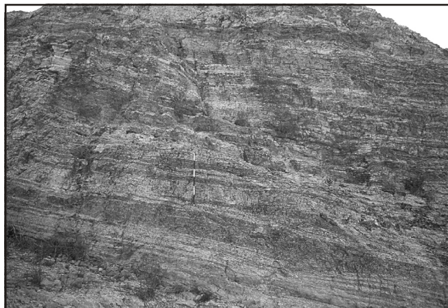
Figure 4. Photograph showing layered mylonitic gneiss. Scale in six-inch divisions.
