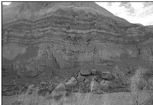
Figure 6. Color banding in clays is more suggestive of diagenetic changes rather than paleosols. Note the concentration of banding toward the surface, with the color banding fading with depth. Perhaps the color banding is a weathering phenomenon, more study is required. Photograph from an exposure along Dawson Creek.
