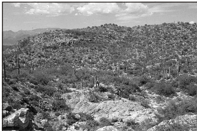
Figure 9. Large hill composed of sedimentary strata that has slumped westward toward the Tucson basin. The strata are contorted as a result of their lateral displacement.
