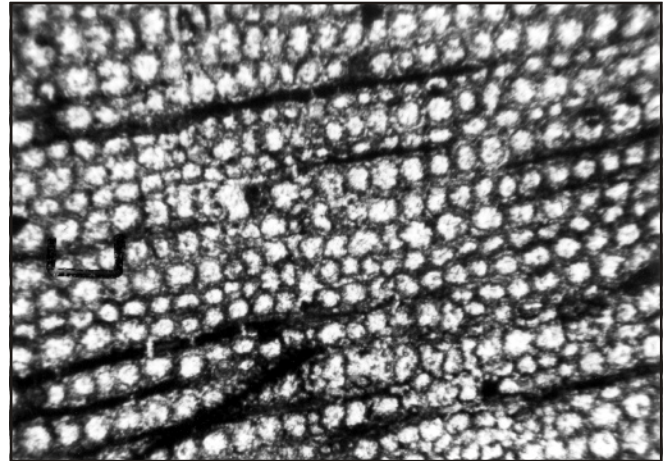
Figure 3. Thin section of fossil silicified gymnosperm wood from bentonite clay mound, south of park Road, Dawson Creek Region, Big Bend National Park. Note the many light-colored tracheids and the darker, radially arranged ray parenchyma cells. Scale bar is 100 micrometers ( \mu\text{m} ).
