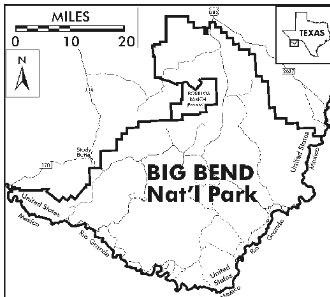
Figure 1. The investigation of petrified plant material and paleosols covered most of Big Bend National Park.
