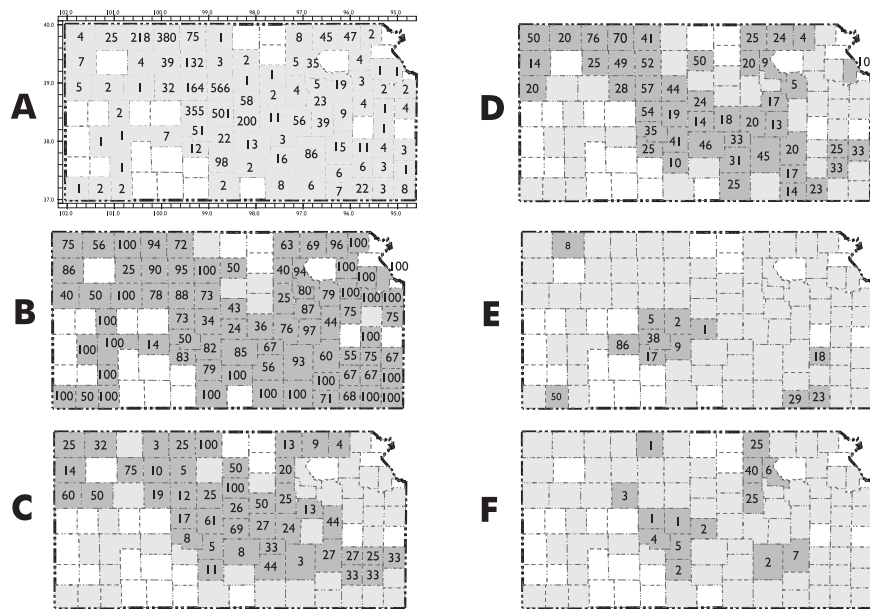
Figure 12. Basement lithology by county based on well penetrations. A = base map showing number of wells penetrating basement drilled in each county prior to 1985, B = percentage of wells encountering granite or granite wash, C = percentage of wells encountering metamorphic rocks, D = percentage of wells encountering granite wash, E = percentage of wells encountering rhyolite, F = percentage of wells encountering basic igneous rocks. Data from Cole and Watney (1985).
