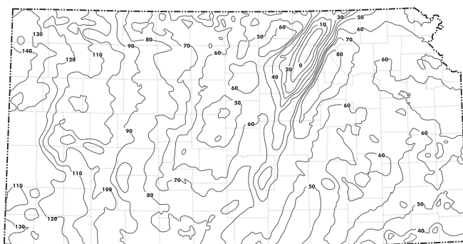
Figure 9. Bouguer Anomaly Map. After Xia et al. (1993).
