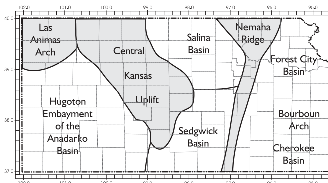
Figure 2. Basement features of Kansas after Zeller (1968).
