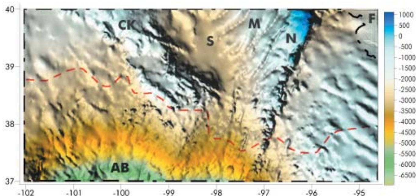
Figure 8. Precambrian basement surface showing 3-D elevation. AB = Anadarko Basin, CK = Central Kansas uplift, S = Salina Basin, M = Midcontinent Rift, N = Nemaha Uplift, F = Forest City Basin. Red dashed line shows boundary between northern and southern terranes according to Xia et al. (1995). Map axes are labeled in accordance with the unprojected latitude/longitude grid used. Based on Bickford et al. (1979).
