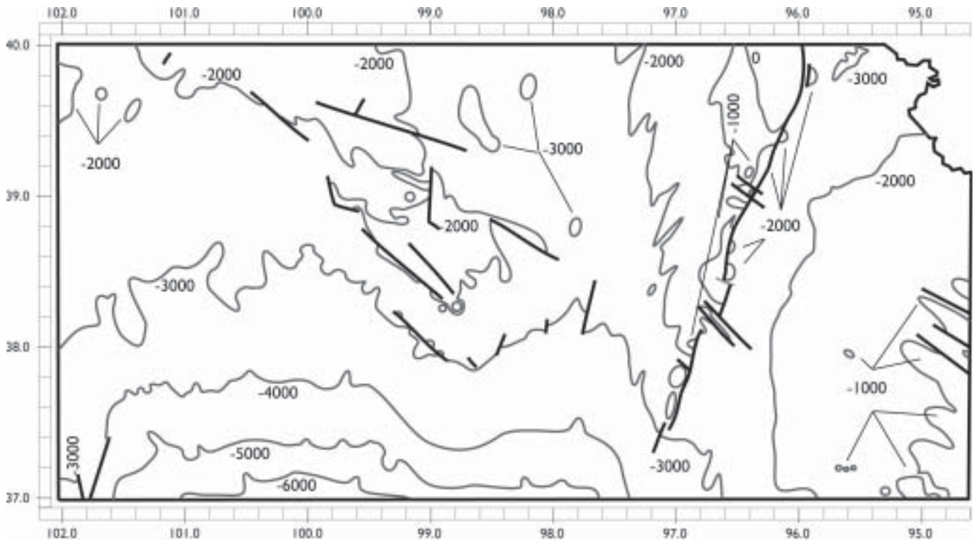
Figure 7. Precambrian subcrop structural surface elevations. After Cole (1976) and Bickford et al. (1979).
