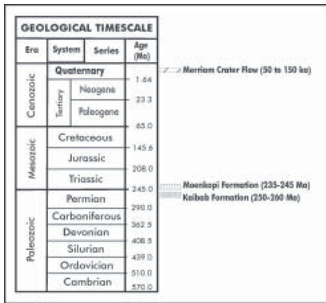
Figure 4. Generalized geologic timescale showing the chronostratigraphic position of the stratigraphic layers found exposed at Grand Falls. The gap between the Kaibab/Moenkopi and the overlying Merriam basalt is missing from the rock record. Are rocks missing because of erosion or were they never deposited? Either way, the existing strata should present evidence showing the passage of millions of years of time if that much time has actually elapsed.
