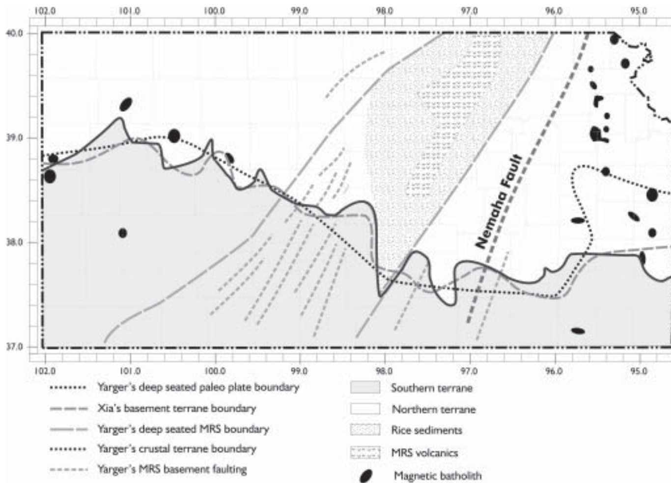
Figure 11. Basement terrane boundaries in Kansas. Modified from Yarger (1983) and Xia (1995).
