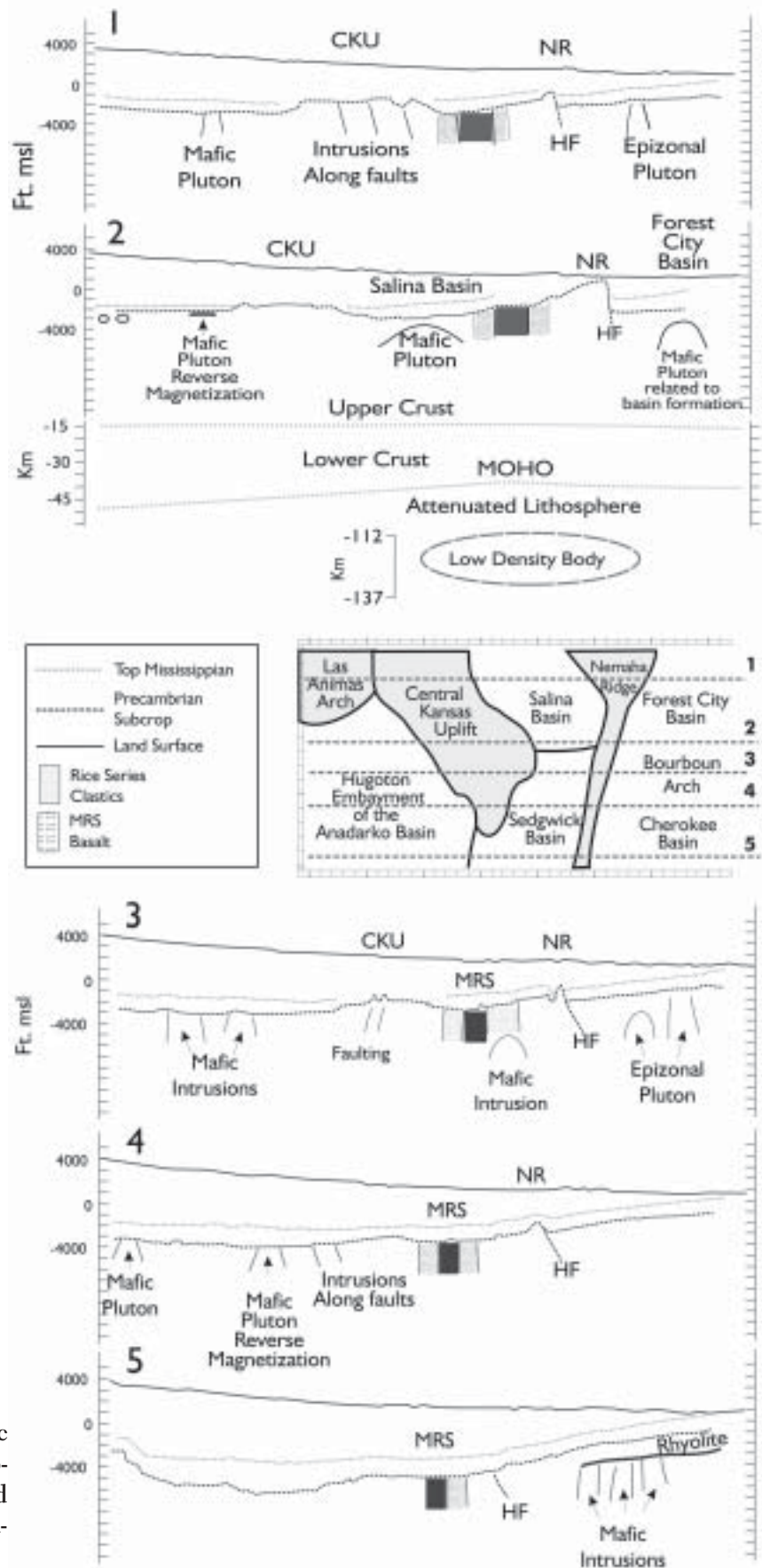
Figure 10. Cross sections of the Phanerozoic cover of Kansas. CKU is Central Kansas Uplift, MRS is Midcontinent Rift System, and NR is Nemaha Ridge. After unreferenced Kansas Geological Society publication.
