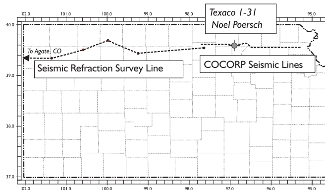
Figure 3. Location of Texaco #1 Noel Poersch well, COCORP seismic reflectionline, and Kansas Geological Survey seismic refraction line. After Berendsen et al. (1988) and Steeples and Miller (1989).
