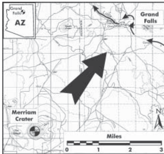
Figure 2. Topographic map showing the relationship between Merriam Crater and the lava flow that blocked the Little Colorado River creating Grand Falls. Modified United States Geological Survey Flagstaff, Arizona Topographic Quadrangle.
