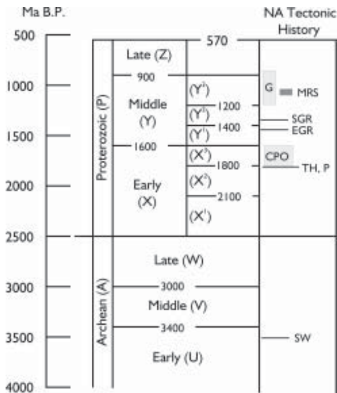
Figure 4. Precambrian time scale with elements of North America's uniformitarian tectonic history. SW is the Superior/Wyoming province, TH is the Trans-Hudson orogen, P is the Penokean orogen, CPO is the Central Plains Orogen, EGR is the Eastern Granite-Rhyolite province, SGR is the Southern Granite-Rhyolite province, G is the Grenville orogeny and MRS is the Midcontinent Rift System. The timescale is from Reed (1993).
