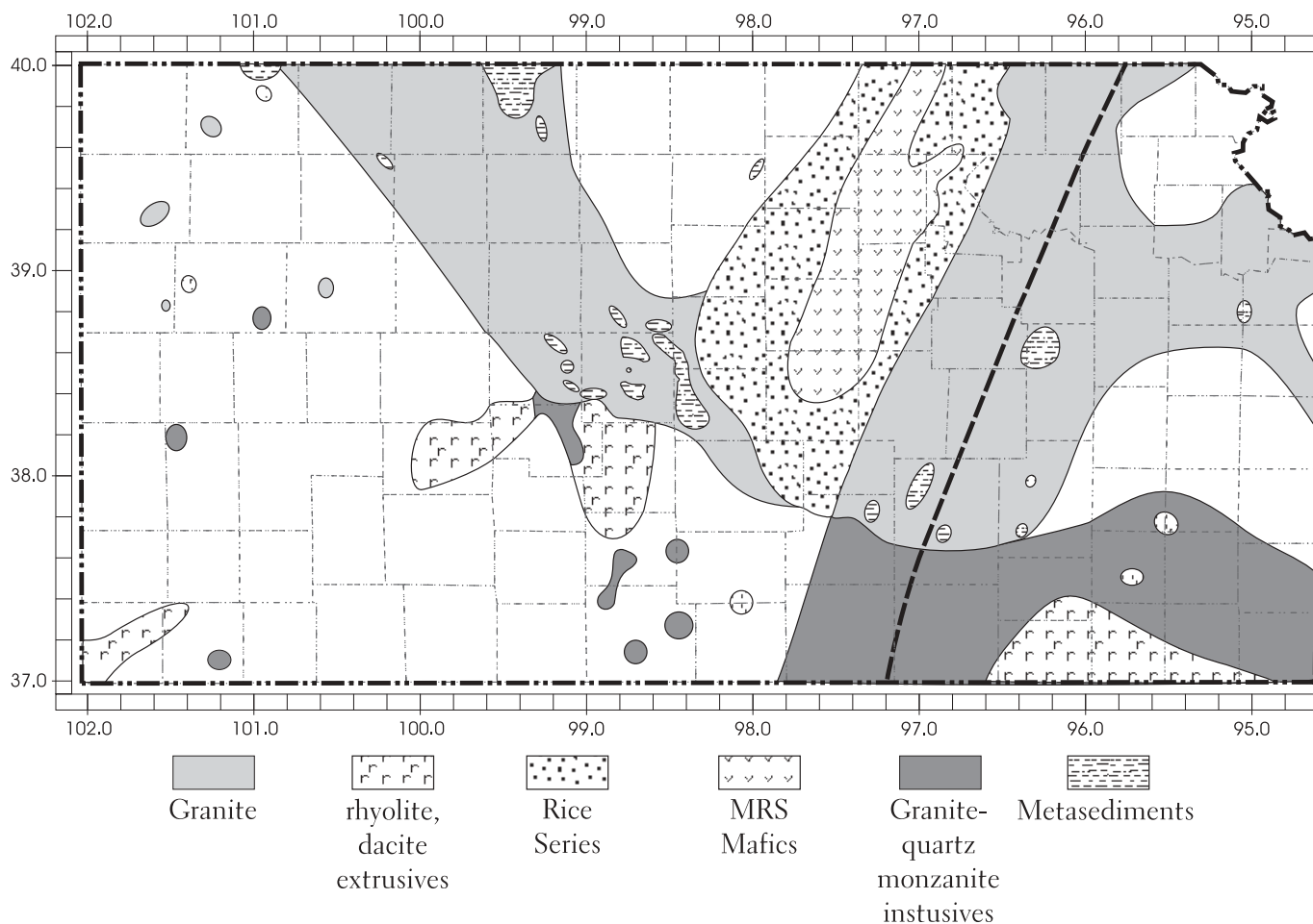
Figure 6. Precambrian subcrop (lithology) in Kansas. From Bickford et al. (1979).
