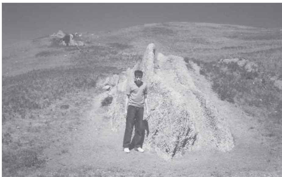
Figure 2. Outcrops of steeply southwest-dipping shell hash limestone (coquina) on rolling terrain devoid of glacial evidences. According to the traditional view of earth history, this region experienced many thousands of years of glaciation.
