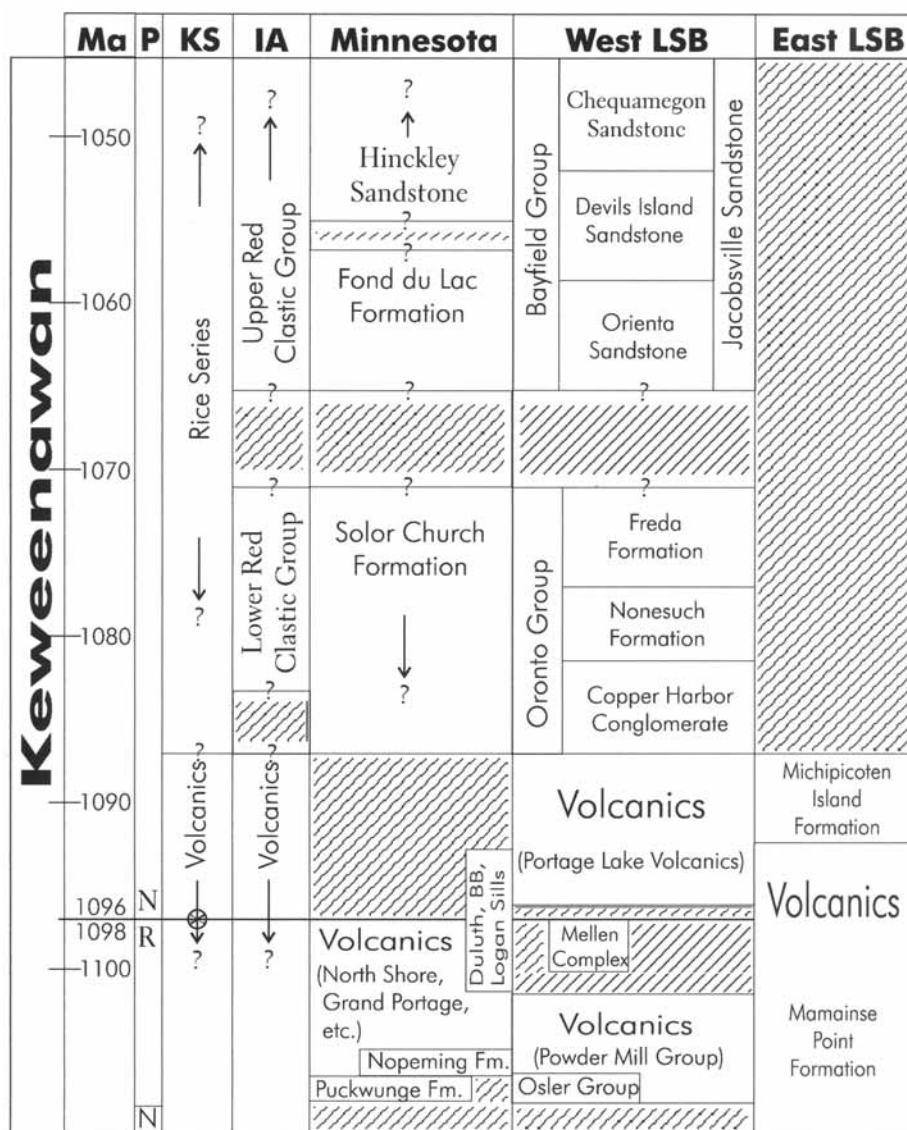
Figure 1. Stratigraphic Chart of Proterozoic Midcontinent Rift Rocks in central North America. From Reed (2000). “P” is magnetic polarity, KS is Kansas, IA is Iowa, and “LSB” is Lake Superior Basin.
