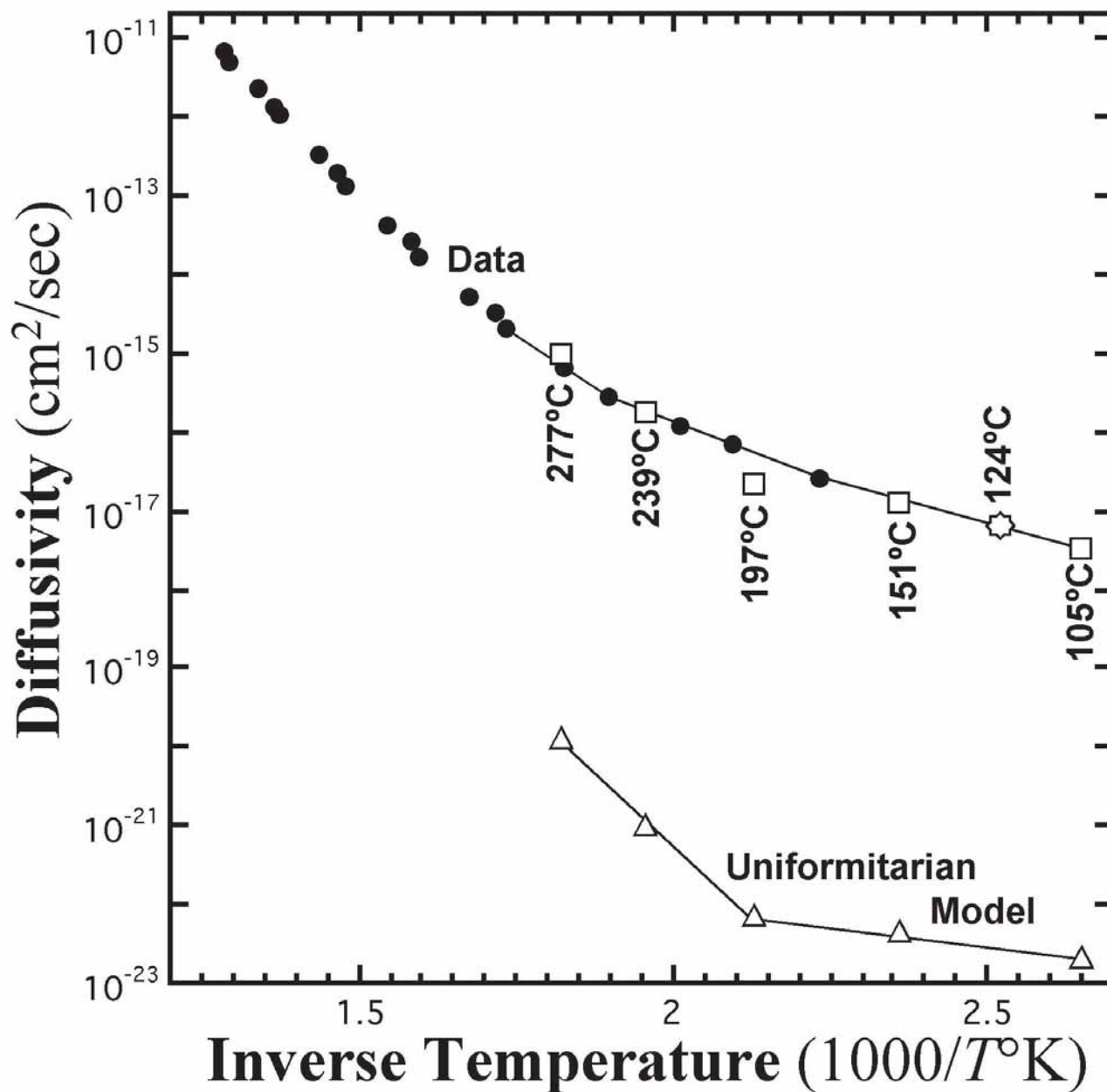
Figure 8. Figure 6 with lines redrawn in accordance with the new (2003) data. Squares with temperatures below them are the diffusivities we predicted in 2000 on the basis of Gentry's reported retentions (Table I, samples 1-5) and an age of 6,000 years. The star with "124° C" above it is the diffusivity required by our new retention datum (Table I, sample 2003, and page 9) and a 6,000-year age.
