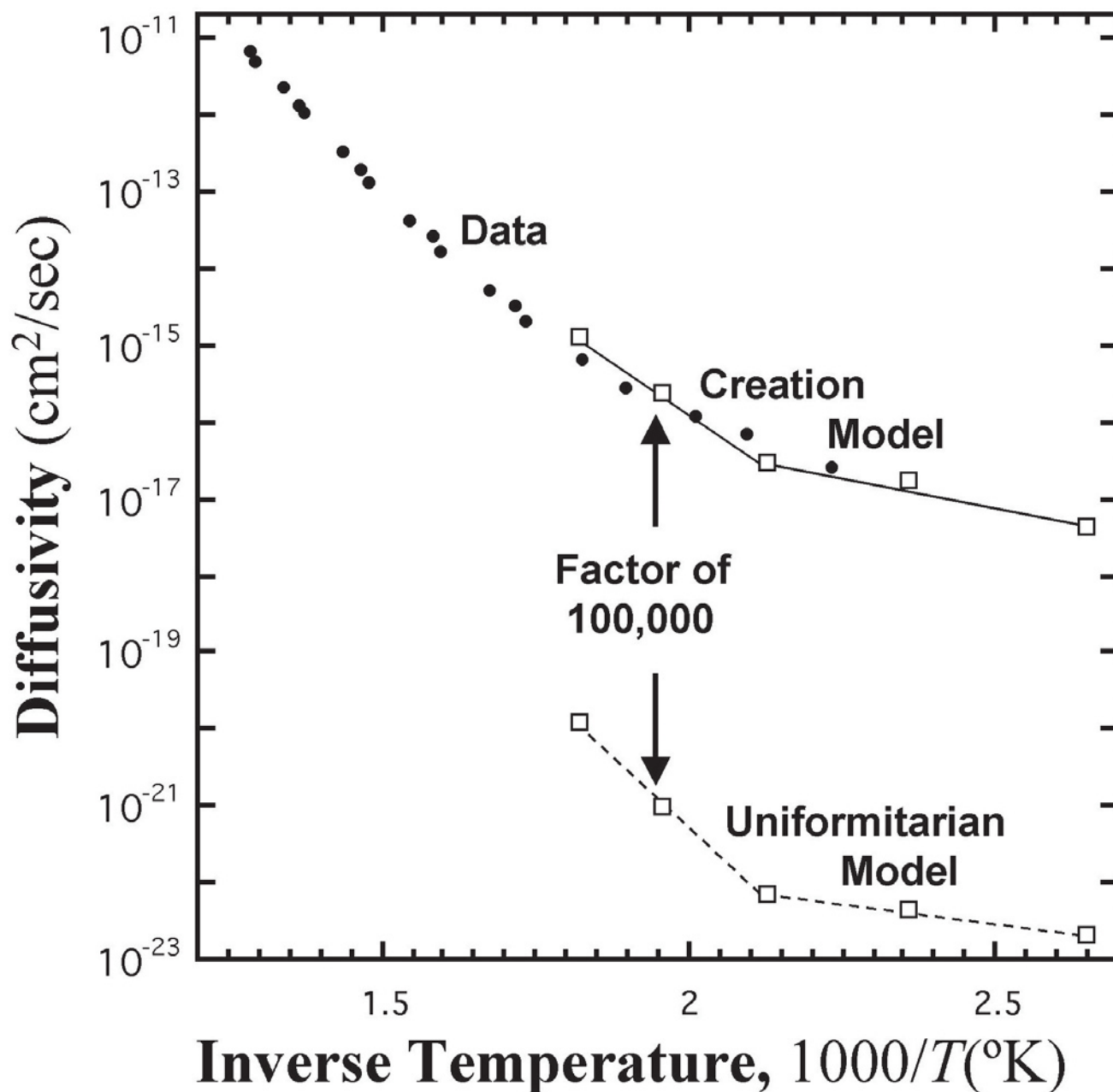
Figure 6. Recent (2003) zircon diffusion rate data compared with the Creation and Uniformitarian models shown in Figure 4.
