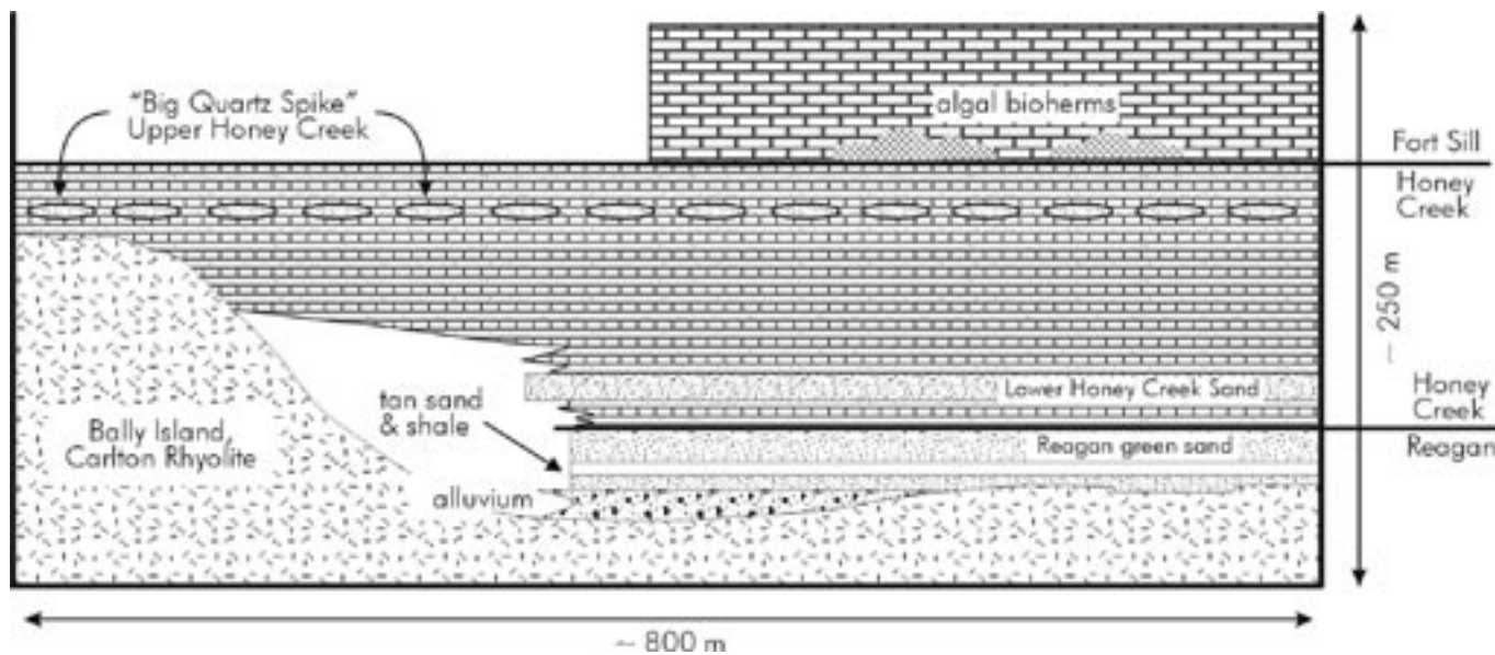
Figure 7. Cross section of the Timbered Hills Group at Bally's Island in the Slick Hills. See Figure 5 for location. Modified from Donovan and Burchett (2000).
