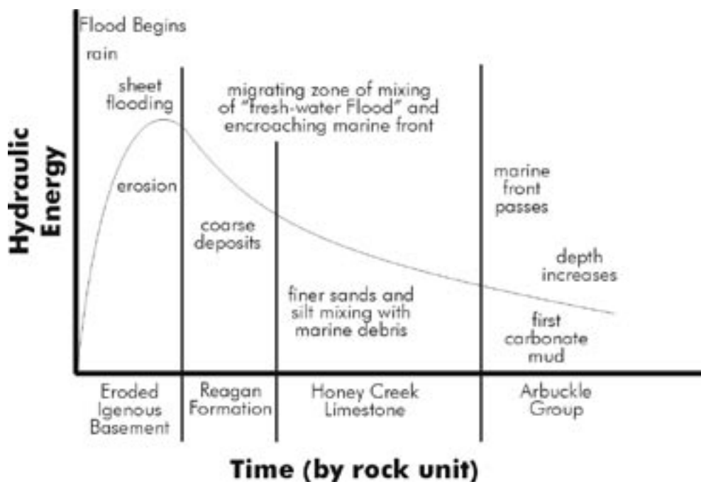
Figure 11. A paleohydraulic curve of the early Flood shows the expected sequence of erosion, followed by deposition of the Timbered Hills Group, as energy increased rapidly at the onset of the Flood and then decreased as the marine front moved across Oklahoma.
