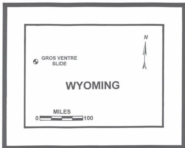
Figure 7. Location of the Gros Ventre Slide in Wyoming. Drawing by Mary Elizabeth Akridge.
