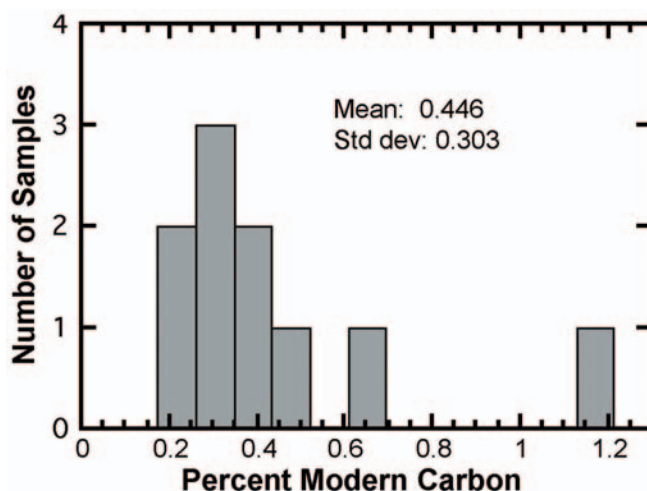
Figure 8. Distribution of ^{14}\text{C} values for the four \text{CO}_2 gas wells.
