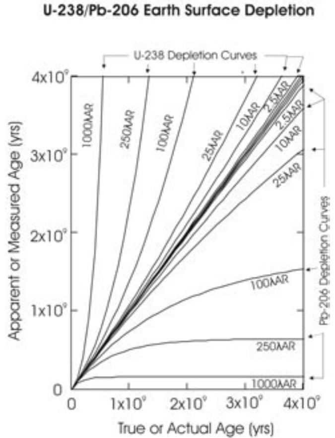
Figure 6. Measured age versus the actual age near the earth's surface where depletion of the parent or daughter dominates. The curves above and below the diagonal represent depletion of U-238 and Pb-206, respectively. The value \lambda AR is selected as the rock atomic loss constant equal to the decay constant of Sm-147 (half life = 106 billion years). Just a little transport of dating isotopes can distort the actual age. Plots for other dating isotopes look similar to this.
