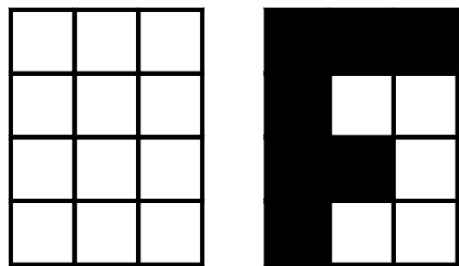
Figure 4. A letter ‘F’ image on the 12 pixels shown in Figure 3.
