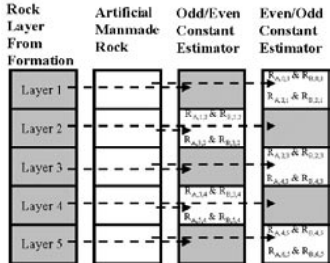
Figure 3. The rock layer atomic loss constant ( R ) can be measured for a formation where one-dimensional transport is believed to have occurred by separating the layers and stacking native and artificial rock layers under heat, fluid, pressure so nuclide transport can occur for an extended period of time and R can be estimated for the surfaces.
