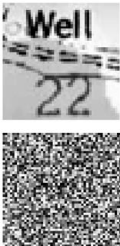
Figure 2. 50 by 50 pixel image of a small section of a topographic map. The correctly digitized (scanned) image is shown in (a), while the scrambled pixels shown in (b) represent one redistribution of the 2500! ( 1.63 \times 10^{7411} ) possible permutations of the pixels for this image. 50 by 50 pixels is roughly 1/6^{\text{th}} of the foveal FOV for human eyes.
