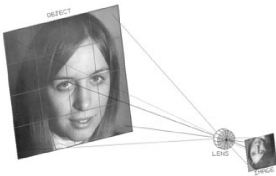
Figure 1. An object scene is viewed by a lens and an inverted image is formed in the focal plane of the lens. In a digital camera, a grid of light-sensitive elements (pixels) divides the image into a matrix. In the human retina, the matrix of rods and cones must be correctly connected to the brain in order for the image to be faithfully restored.
