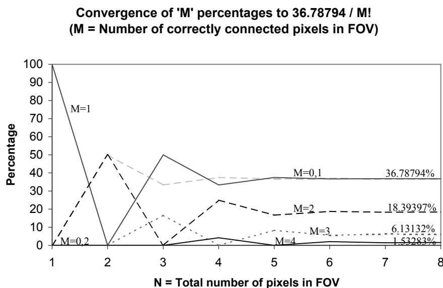
Figure 8. For 1-4 correctly connected pixels (M), the percentages of the pixel-connection permutations quickly become constant with increasing numbers of pixels in the FOV. The same trends apply to values of M > 4 where the percentages converge to 36.78794/M! .
