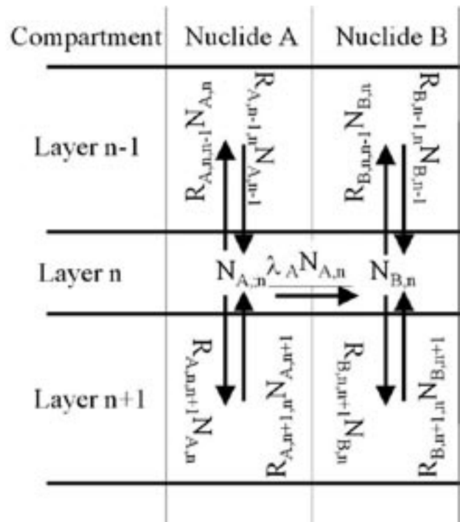
Figure 2. The transport processes in a one-dimensional layered system bounded above by the atmosphere and below by additional layers of rock. Nuclide A can leave layer n by three routes (top, bottom and decay of A) and come into the system by two routes (top and bottom). Nuclide B can leave by two routes (top and bottom) and enter by three routes (top, bottom & decay of A).
