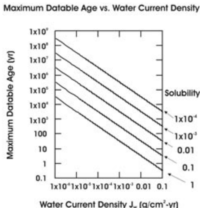
Figure 8. The maximum datable age for a rock sample is strongly dependent on the solubility of the dating isotopes and the water flow through the rock. The graph is for a 100 cm long rock core where the dating isotopes are insoluble (10 -4 g per 100 ml of water) to soluble (1 g per 100 ml of water). Concentration is 1 PPM and density of rock is 3 g/cm 3 . A combination of high concentrations of dating isotopes, long rock cores, low water flow rates, and insoluble dating isotopes are required to achieve maximum datable ages of a billion years. For comparison with the water flow through rock, rainfall in arid regions may be 10 g/cm 2 -yr. A small fraction of this rain penetrating the rock may render the system open.
