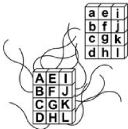
Figure 3. A 12-wire connection example where the same capital letter to lowercase letter is the correct connection, and all others have some level of error.
