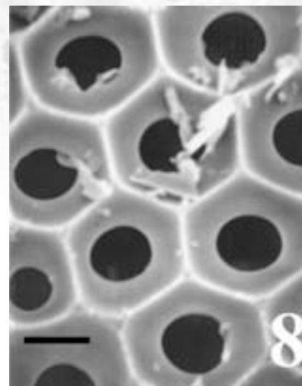
Figure 8. Extreme SEM enlargement image of the area around the large black arrow in Figure 7. Note the intricate, repeating pattern of hexagons and the 2–3 micrometer pores within the diatom frustule wall. This greater complexity of detail seen at higher and higher magnification in a diatom frustule wall crushes the concept of chance as its means of origins. It supports creation by a Creator who possesses limitless skill. Scale bar is 2.3 micrometers, with a magnification of 12,000X.
