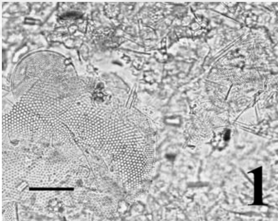
Figure 1. A speck of diatomite from the Lompoc deposit in water on a microscope slide shows the tightly compacted nature of the deposit. Some exquisite patterns are still visible in the glass cell walls of diatoms in this light micrograph. The scale bar, lower left, is 50 micrometers.
