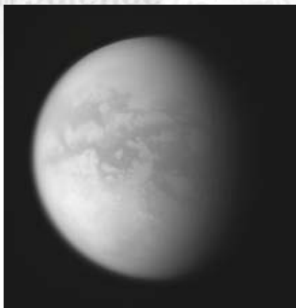
Figure 1. Outbound photo of Titan from Cassini orbiter camera at a distance of 148,000 km. Image scale is 9 km per pixel. Photo courtesy of NASA/JPL/Space Science Institute.
