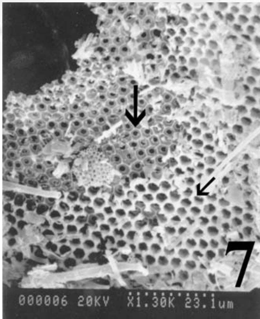
Figure 7. SEM enlargement image of the diatom in Figure 6. Note the upper layer (small black arrow) and the lower layer (large black arrow) of the frustule wall. Such intricacy is a tribute to the divine Designer. Dotted scale bar is 23 micrometers.
