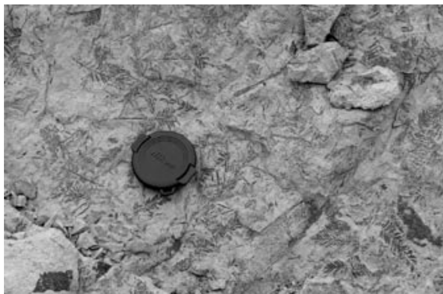
Figure 14. Coalified leaves and needles showing little if any decay. Lens cap for scale.
