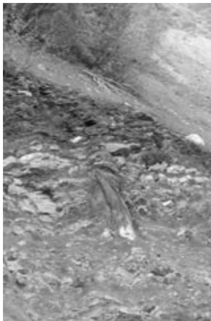
Figure 9. Polystrate tree from the fourth mine with about 3 m exposed.
