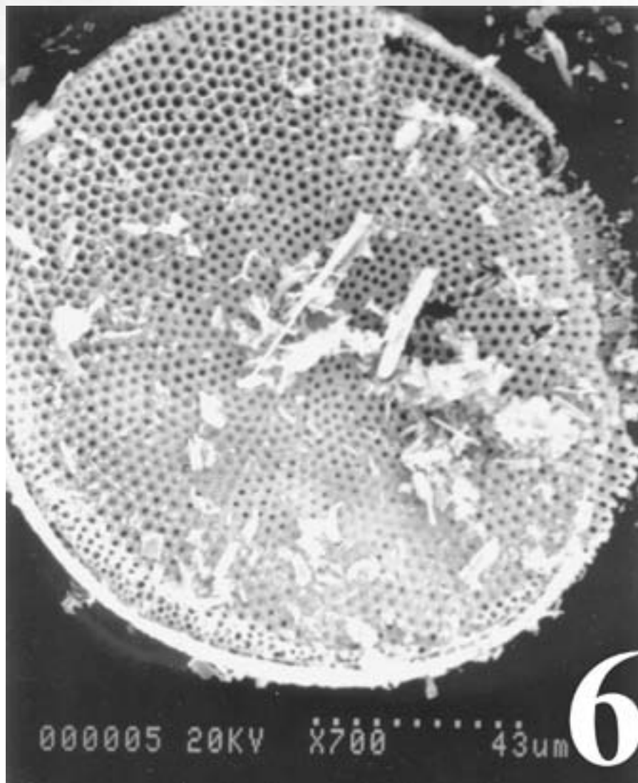
Figure 6. SEM image of an individual centric diatom from Lompoc diatomite. Although part of the frustule (right side) has cracked away, the detail visible in this tiny object is overwhelming! Dotted scale bar is 43 micrometers.
