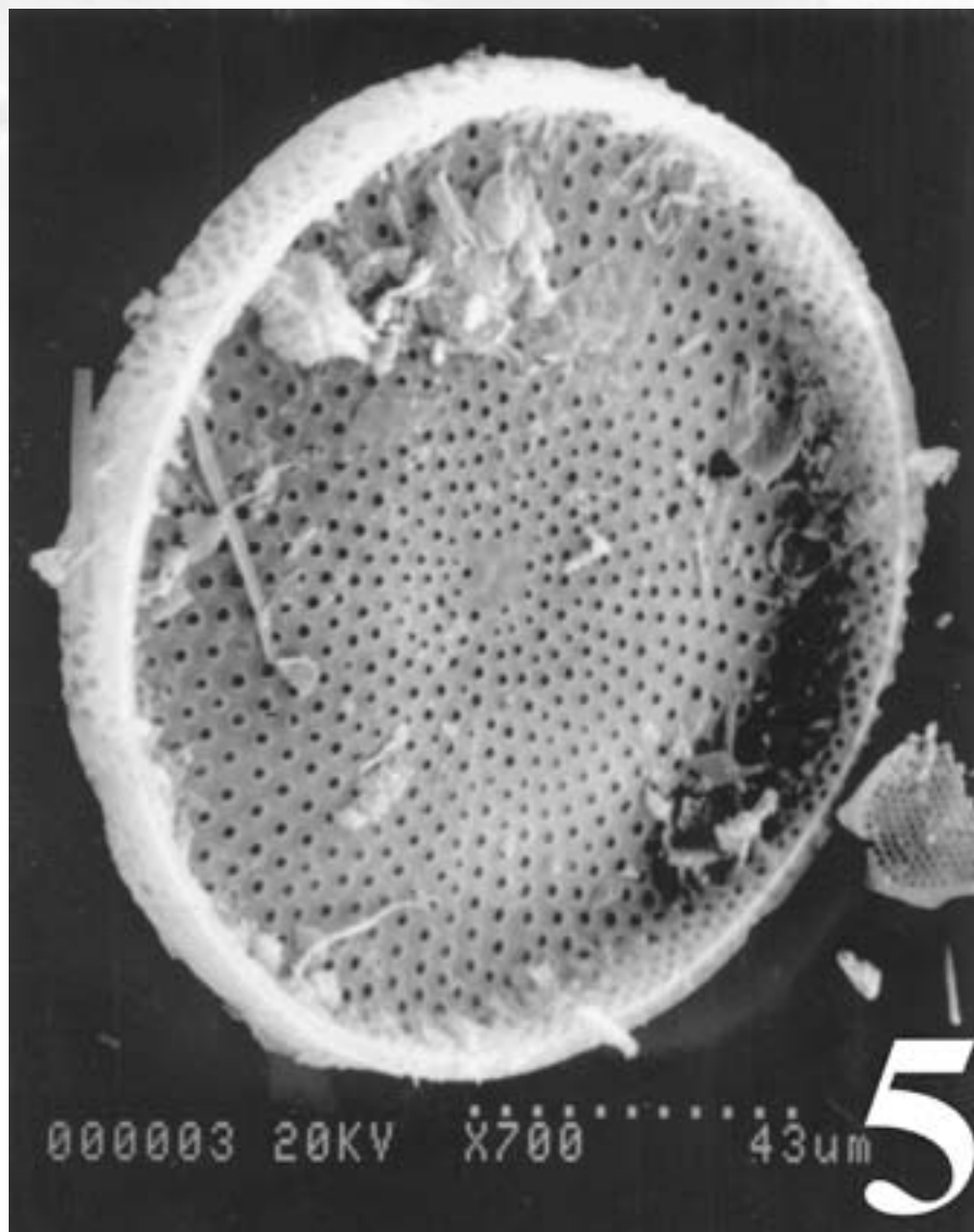
Figure 5. SEM image of an individual centric diatom separated from the tightly compacted Lompoc diatomite and mounted. Note that this circular diatom frustule shows even greater detail than the one seen in Figures 3 and 4. Dotted scale bar is 43 micrometers.
