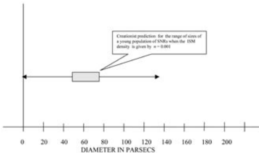
Figure 3. This box chart represents the creationist predictions for the range of sizes of SNRs of average expansion characteristics moving through an ISM of density corresponding to n = 0.001 . This density has been estimated as applying to 70% of The ISM.
