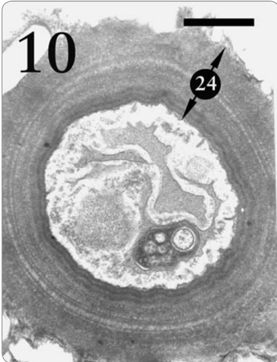
Figure 10. Fungus cell from the medulla region of Xanthoparmelia sp. It is quite advantageous for lichen fungal cells in the medulla tissue to possess thick walls (24) where support is required (Armitage and Howe, 2006, pp. 258, 260). The same fungus species makes much thinner cell walls in the algal zone (see Figure 7, number “14” at the top) where absorption of photosynthetic products is a priority. Magnification 15,000X, scale bar 1 micrometer.
