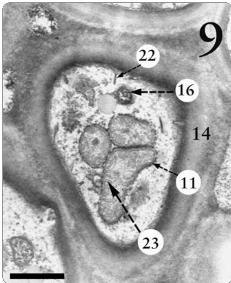
Figure 9. A cell of the mycobiont of Candelariella sp. Invaginations of the plasmalemma (22) greatly increase the membrane surface area, thus fostering added contact necessary for various functions. In the center of the cell are three mitochondria (11). Folds of the mitochondrial inner membrane (23) contain a host of enzymes required for the respiratory synthesis of ATP, which is sometimes called the high energy “currency” of the cell. Several other items labeled in previous figures are numbered here as well. Magnification is at 14,000X, and the scale bar is 2 micrometers.
