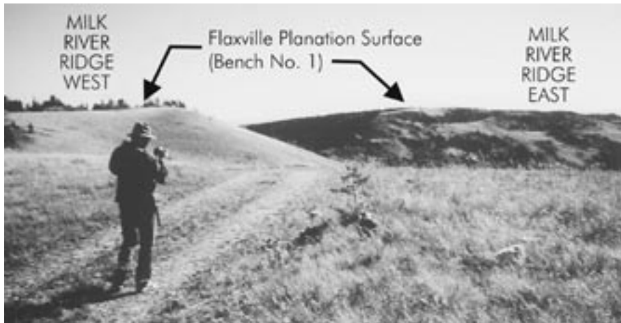
Figure 16. East end of Milk River Ridge from west end of ridge.
