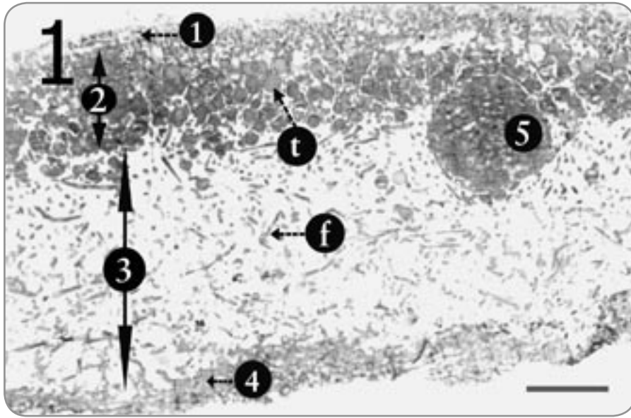
Figure 1. A brightfield photomicrograph of a cross section of a typical foliose lichen Xanthoparmelia sp. with its tissue zones labeled. The tissues are: upper cortex (1), algal layer (2), medulla (3), and lower cortex (4). Area (5) appears to be a developing reproductive structure called an apothecium . A Trebouxia cell in the algal layer is labeled "t," while item "f" is a fungus hypha in the medulla. Lichens are thought to be very distant taxonomically from flowering plants, yet many features found in the tissues of plant leaves are duplicated here in a very generalized fashion (Armitage and Howe, 2004; 2006). A mycobiont produces a complex thallus like this only when it grows with its phycobiont. The same fungus by itself builds no such edifice. This suggests intelligent design. The scale bar is 60 micrometers, and the magnification is 2,000X.
