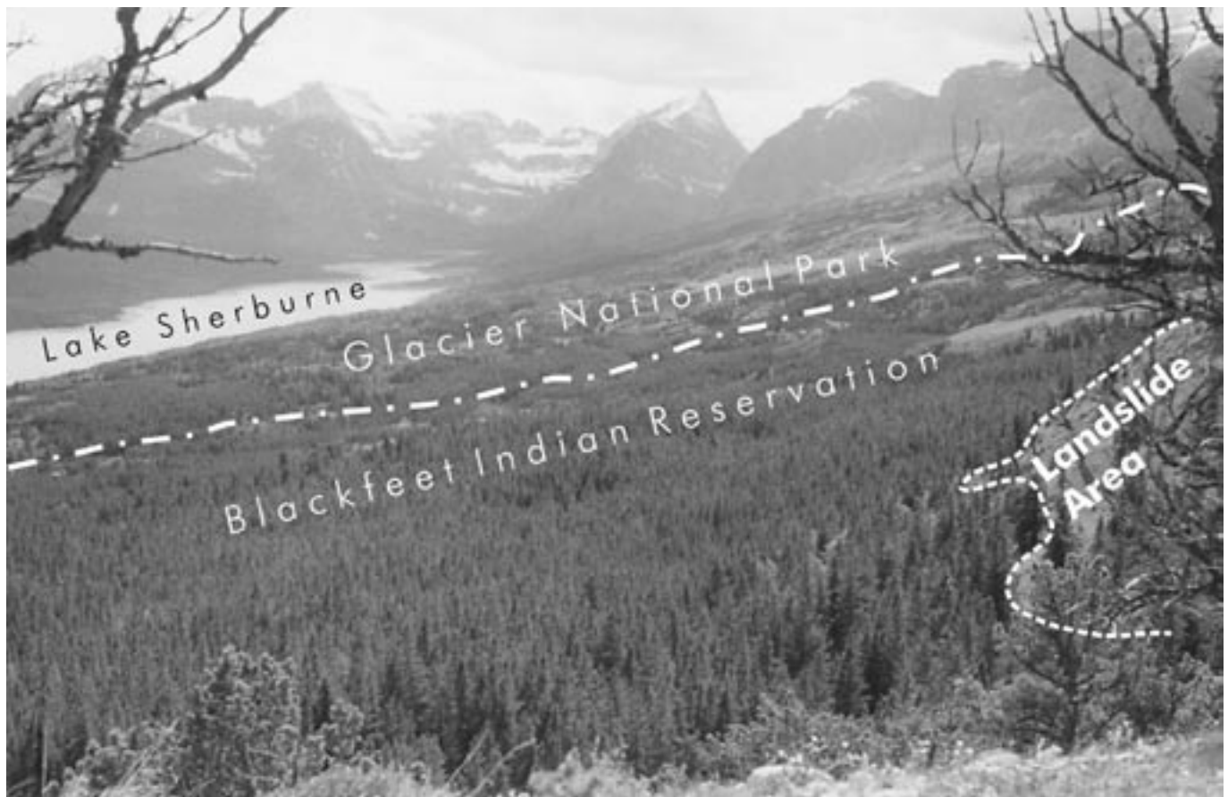
Figure 17. View west along south side of Swiftcurrent Ridge showing landslide area.
