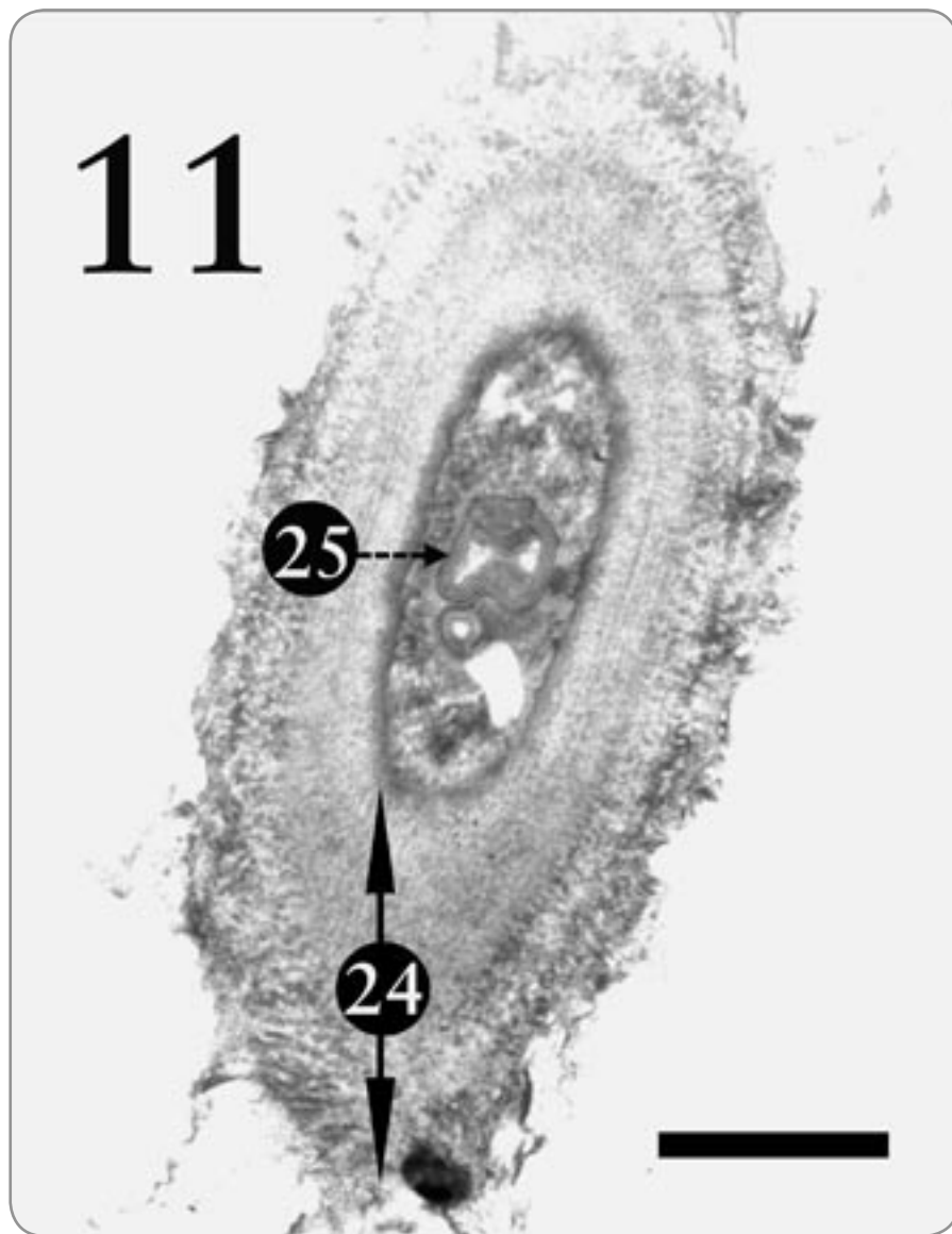
Figure 11. A cell from the mycobiont in the medulla tissue of the same lichen as the previous figure, Xanthoparmelia sp. In the medulla, the lichen fungus ordinarily has a thick, multilayered cell wall (24), enabling the medulla to supply support inside the lichen. A large structure seen here and a smaller one too (25) resemble the myelin-like bodies photographed by Peveling (1973, p. 158) and by Jacobs and Ahmadjian (1969). Myelin-like bodies will be discussed in the forthcoming second part of this article. Note its several layers, which resemble a myelin sheath seen in animal neurons. The magnification here is 12,000X with a scale bar of 2 micrometers.
