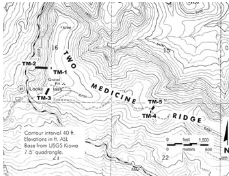
Figure 2. Two Medicine Ridge Sample Map.
