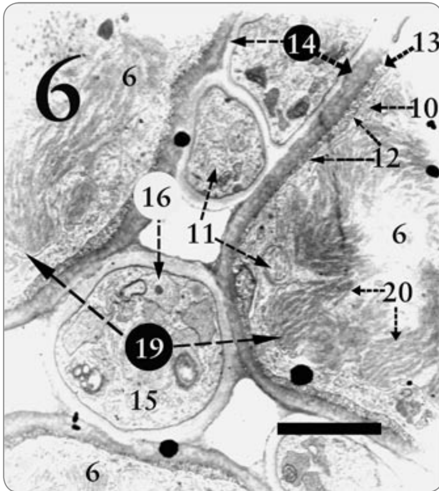
Figure 6. Three Trebouxia phycobiont cells in close contact with four fungal cells. Thylacoid membranes (20) can be seen here in the lichen Caloplaca sp. Some of the features labeled and identified in previous figures are numbered here as well. Magnification is 11,000 X, and the scale bar is 5 micrometers.
