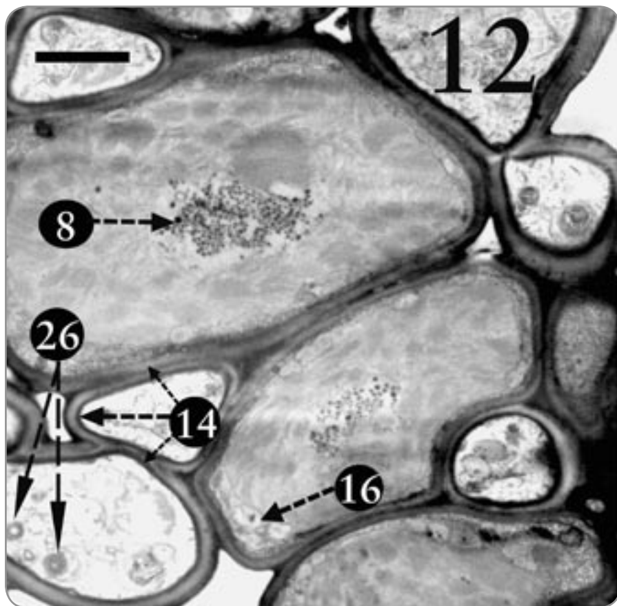
Figure 12. Both mycobiont and phycobiont cells from the algal zone of Candelariella sp.
