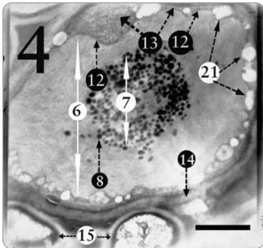
Figure 4. A cell of the phycobiont Trebouxia sp. from the algal zone of the lichen Candelariella sp. [Note: Candelariella is the same yellow-orange lichen that we mistakenly called Candelilaria in our previous articles (Armitage and Howe 2004; 2006), and correctly identified in Howe and Armitage, 2003]. In addition to the storage layer (13) located just outside the plasmalemma (12), many white storage areas can be observed (21) at the outer edge of the cytoplasm. Pyrenoglobuli (8), which store lipids, are also present in the pyrenoid of the chloroplast. At some locations several pyrenoglobuli are arranged in an orderly line because of their attachment to the thylacoid membranes of the pyrenoid. Numbers for other subcellular particles are as on the previous figures, (6) chloroplast, (7) pyrenoid, and (14) cell wall. Two mycobiont cells (15) are closely appressed to the alga. The three different storage systems seen here enable lichens to thrive despite long periods of unfavorable climate. The magnification is 10,000X, and the scale bar is 6 micrometers.
