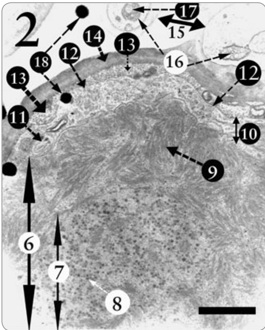
Figure 2. A transmission electron microscope (TEM) photograph of Trebouxia sp., a green alga present in many different lichens, and two accompanying fungal cells from the algal zone of the lichen Caloplaca sp. This figure, and all those which follow, are TEM photographs. The numbered visible items here are a cell of the phycobiont Trebouxia sp.: chloroplast (6), pyrenoid inside chloroplast (7), pyrenoglobuli (8), thylacoid membranes inside the chloroplast (9), cytoplasm (10), mitochondria (11), cytoplasmic membrane (usually called the plasmalemma ) (12), storage region just outside the plasma lemma (13), cell wall (14), cell of the fungus in the Caloplaca lichen (15), nucleus (16), nucleolus (17), and an artifact (18). Dark dots like these on other figures are artifacts as well. The magnification is 11,000X, and the scale bar is 4 micrometers.
