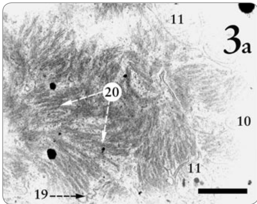
Figure 3a. The chloroplast of a Trebouxia algal cell from the algal zone of Caloplaca sp. The chloroplast of Trebouxia is deeply cleft, forming lobes along its margin (19). Thylacoid membranes of the chloroplast are arranged into grana-like stacks (20), and algal mitochondria (11) are visible in the surrounding cytoplasm (10). The magnification is 14,000X, and the scale bar is 2 micrometers.
