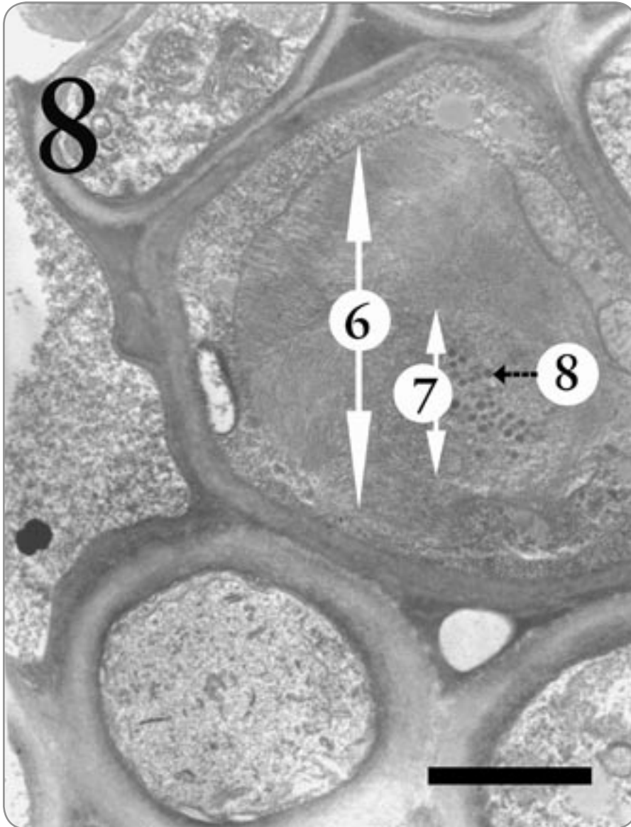
Figure 8. A cell of the green alga Trebouxia from the algal zone of the lichen Candelariella sp. Pyrenoglobuli (8) are visible, attached in an orderly fashion to the thylacoid membranes of the pyrenoid (7). Pyrenoglobuli contain energy-rich lipids and may perform other important tasks, such as supplying water. Magnification is 11,000 X, and scale bar is 5 micrometers.
