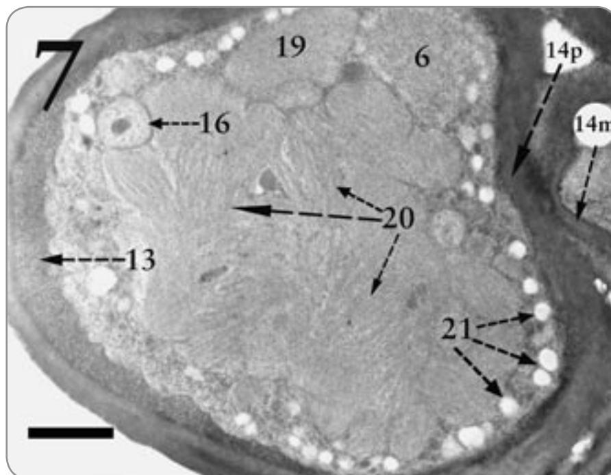
Figure 7. Trebouxia phycobiont cell from the algal zone of the lichen Xanthoparmelia sp. The following features can be easily distinguished: white storage regions in the cytoplasm (21), storage layer between the plasma-lemma and the cell wall (13), a lobe of the large chloroplast (19), nucleus and nucleolus of the Trebouxia cell (16), cell wall of the mycobiont (14m), cell wall of the phycobiont (14p), and the stacks of thylacoid membranes (20). Note above, center, the relatively thin cell walls the mycobiont hypha has here in the algal zone of this lichen and compare to the thick walls it produced in the medulla tissue of the same lichen species— Xanthoparmelia (see caption of Figure 10). These differences enable the fungus to receive photosynthate from nearby algal cells, whereas in the medulla the thicker walls supply support (see Armitage and Howe, 2006, pp. 258, 261). The magnification is 12,000X, and the scale bar is 4 micrometers.
