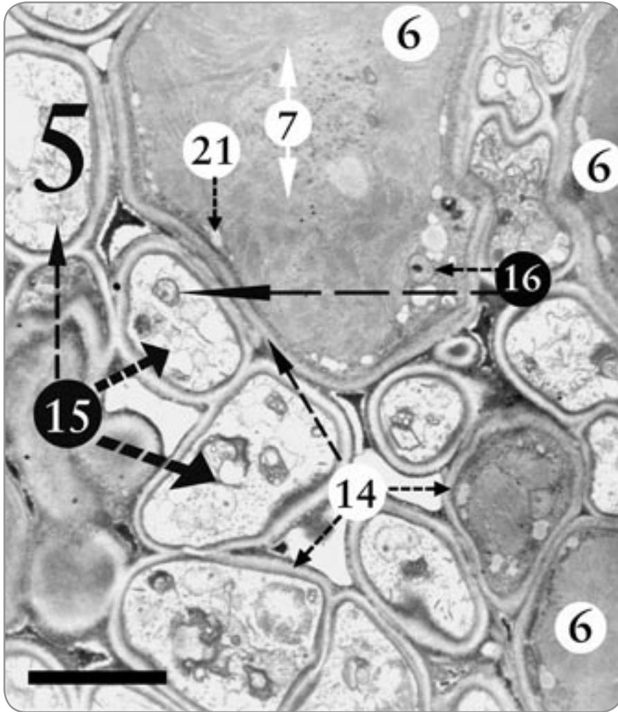
Figure 5. A Trebouxia sp. phycobiont cell surrounded by many fungal cells (15) in the algal zone of Candelariella sp. In this one section, at least 10 fungal cells are seen in close contact with the one algal cell, upper center, where one whole cell and parts of two others are visible (6). Nuclei with nucleoli are evident in various algal and fungal cells (16). Nucleoli store and transport messenger RNA molecules, which in turn encode for the production of proteins. The magnification is 8,000 X, and the scale bar is 10 micrometers.
