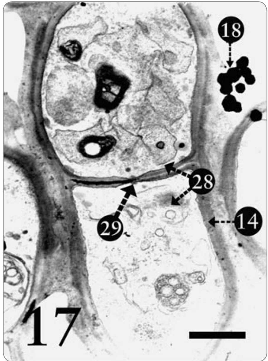
Figure 17. Mycobiont cells of the lichen Caloplaca sp.: magnification 12,000X; the scale bar is 30 micrometers. A perforated septum (28) separates the upper and lower cells (28). The unnumbered hole between them can become clogged by a pluglike structure known as a Woronin body (29). Woronin bodies can plug damaged hyphae, serving to prevent further loss of cytoplasm from the cells. The cytoplasm of the upper cell here is fragmented (as in certain cells of Figure 17), perhaps indicating the synthesis of spores, if this is in fact a developing ascus in an apothecium.
