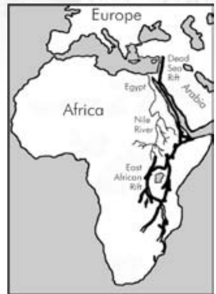
Figure 1. The Great Rift extends over 4,000 miles from southern Africa into Syria.
