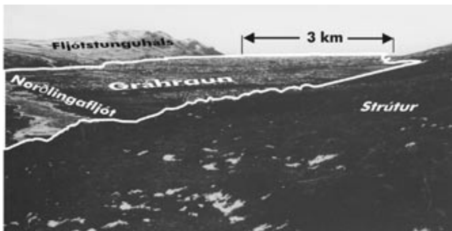
Figure 14. Gráhraun, a pahoehoe flow from ca. A.D. 880. View toward northeast with flow outlined in white. Note that flow fills valley bottom and has diverted the river (Norðlingafjót).
