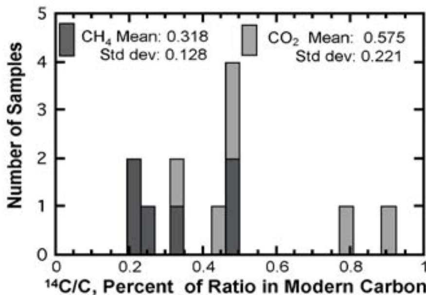
Figure 2. Distribution of 14C values for three Valverde Basin Natural Gas Wells.
