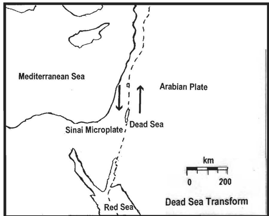
Figure 2. Diagram of the Dead Sea Transform, according to the plate tectonic theory.
