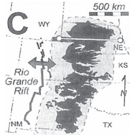
Figure 12. Distribution of the Ogallala Group on the central and southern High Plains of the United States, modified from Thornbury (1965) and Heller et al. (2003). Map shows observed (black) and inferred (shaded) original distribution. White arrows show generalized paleocurrent directions.
