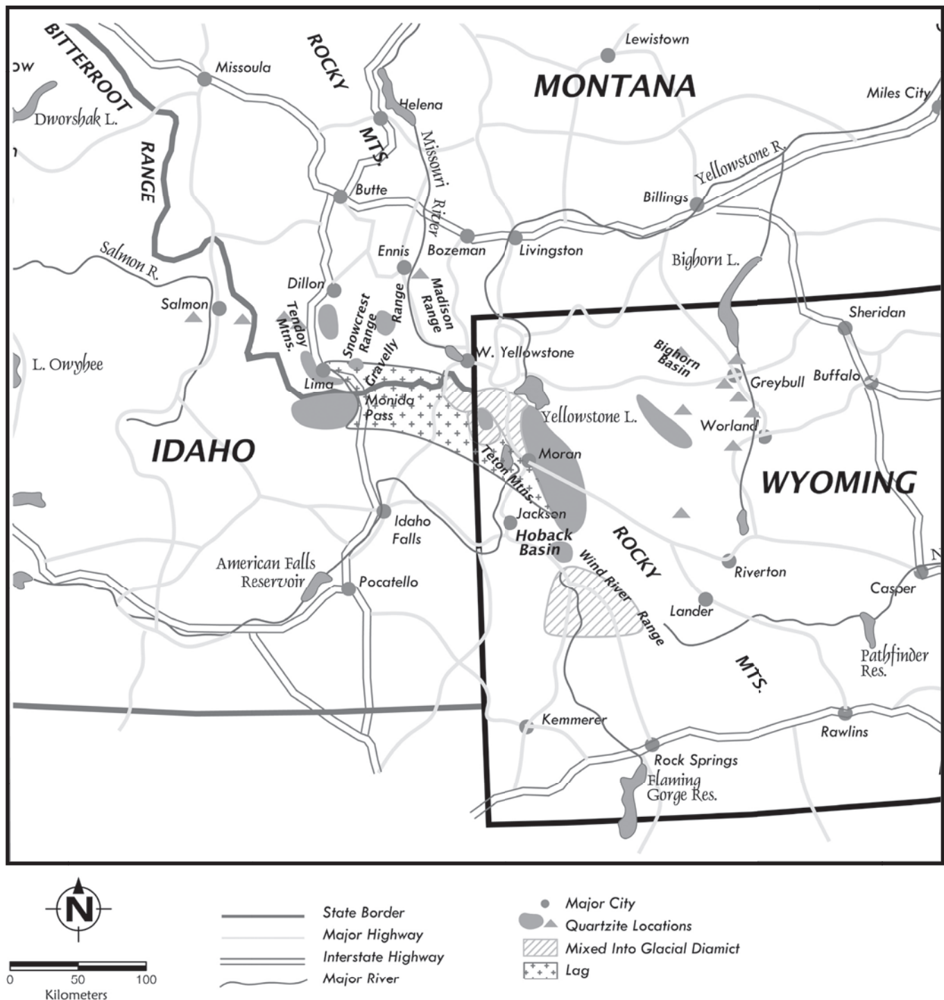
Figure 8. Quartzite gravel locations in southwest Montana, northwest Wyoming, and adjacent Idaho.
