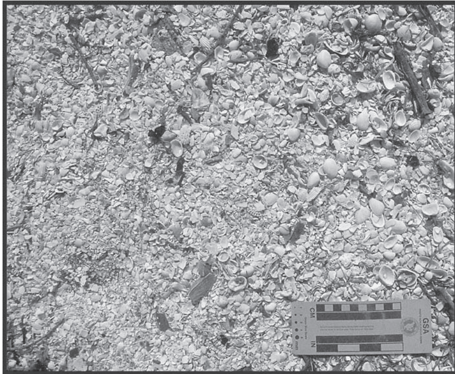
Figure 8. Sanibel Island, on the southwestern side of the Florida Peninsula, is famous to shell collectors. Wave conditions are such that a wide variety of shells are gently washed onshore, and in many cases they are in perfect condition. However, storm waves also serve to batter and break the shells creating a shell hash that if lithified would form a coquina. Such broken shell material can be seen in this image from the beach at Sanibel Island, where whole shells are mixed with broken shells. Note that both the shells and fragments are generally flat-lying. This modern shell deposit is not what is found at Little Stave Creek, so any postulated association between the two locales is inappropriate. Scale in inches and centimeters.
