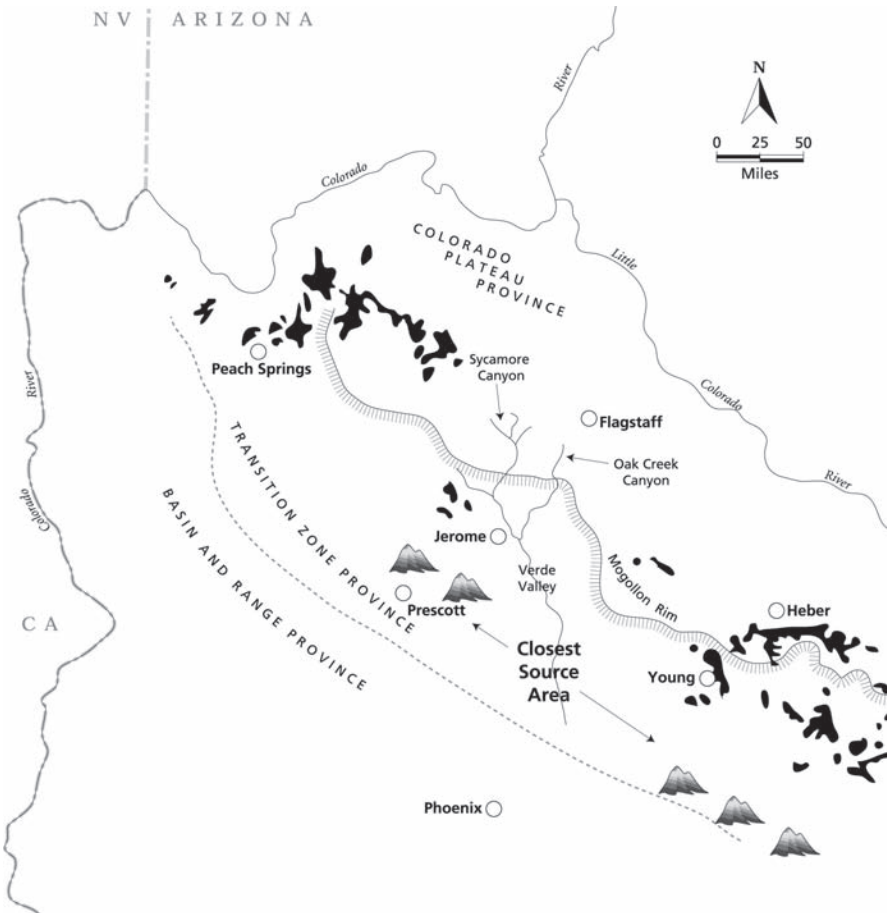
Figure 11. Location of Rim Gravel in Arizona in black. Physiographic provinces of Arizona also are shown. Nearest sources for the Rim Gravel along the northwest and east-central location Mogollon Rim pointed out, but this does not necessarily mean the gravels originated from these locations, since there are many sources to the south and west. Drawn by Mark Wolfe and modified from Elston and Young (1991, Figure 1).
