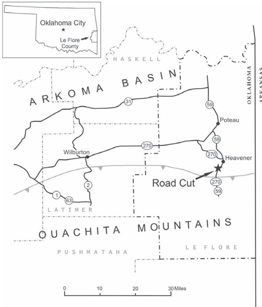
Figure 1. Location of the Heavener roadcut, Le Flore County, Oklahoma (Section 36 of Township 5N and Range 25E, NW, SE, NW) just north of the Choptaw thrust fault, separating the Ouachita Mountains and the Arkoma Basin.
