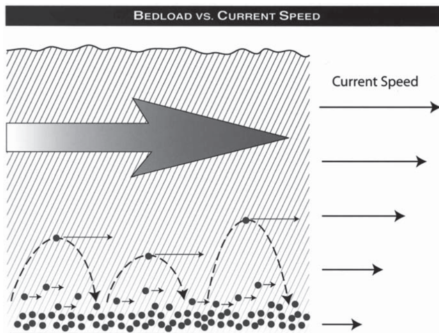
Figure 14. Schematic of turbulent gravel transport in high velocity water. The large rocks are dragged along the bottom as bedload, while the small- to medium-sized rocks are briefly carried up into suspension before crashing back down into the bedload. Drawing by Mark Wolfe.
