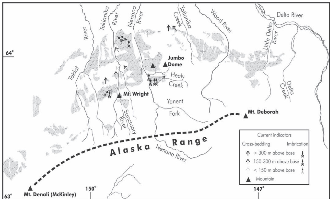
Figure 2. Map of the Nenana Gravel outcrops with paleocurrent directions. Modified from Thom (2000, p. 31).
