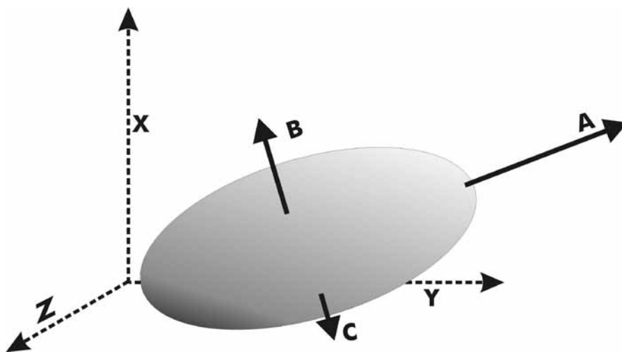
Figure 8. Simple illustration of application of eigenvector analysis: orientation of clasts (individual rocks) in Cartesian coordinates ( x,y,z ) can be described by three vectors aligned with the A-, B-, and C-axes (longest to shortest dimensions, respectively, of the clast). Eigenvector analysis provides a computational method to find which possible combination of orthogonal vectors produces the maximum and minimum axes (and thus mutually perpendicular third axis) of the rock. This same method can be used for many other types of data.
