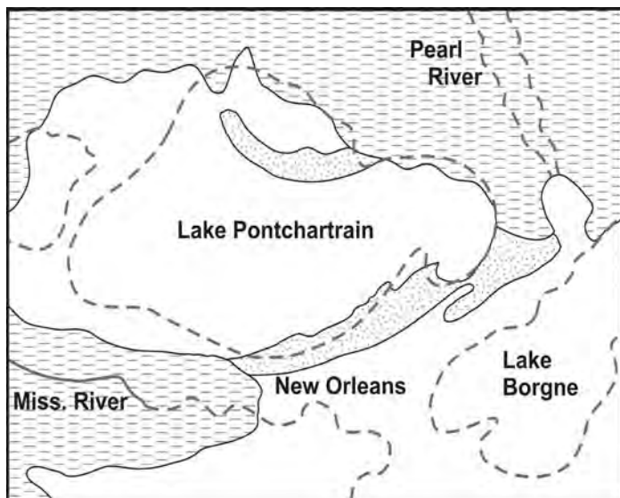
Figure 2 ( left ). Probable configuration of Pine Island Beach Sand in relationship to land and sea in 4,000 BP. Two sand spits developed from east-west longshore currents. The northern one is now under Lake Pontchartrain, and the second underlies much of New Orleans and St. Bernard Parish. After Nelson and Leclair (2006, figure 2).
