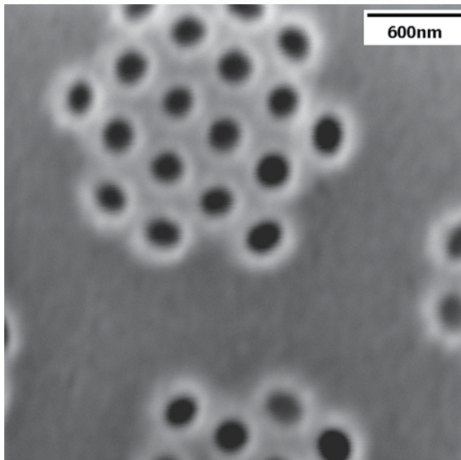
Figure 4. SEM photo of a portion of a centric diatom frustule exhibiting clusters of pores. Magnification 25,000X. Scale bar = 600nm. Pore size = 150nm.
