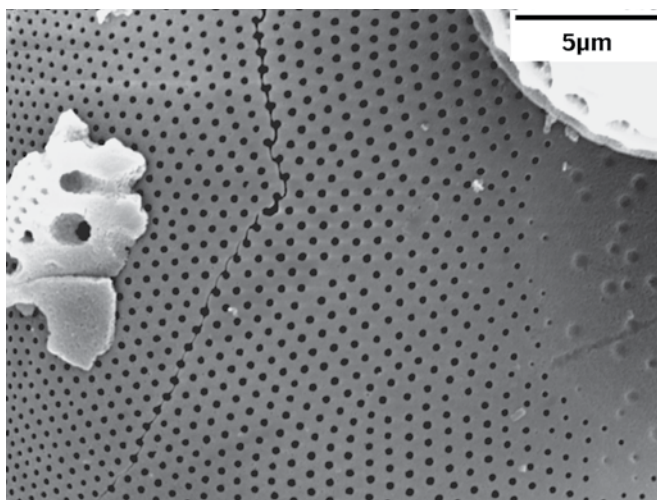
Figure 5. SEM photo of a portion of a centric diatom frustule exhibiting a lattice of pores. Magnification 5,000X. Scale bar = 5 microns.
