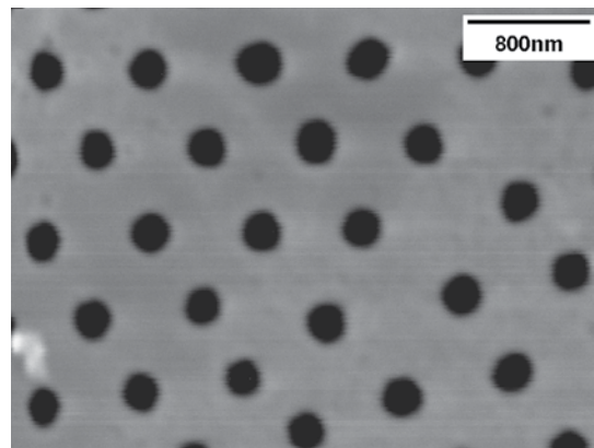
Figure 7. SEM photo of a portion of a centric diatom frustule exhibiting lattice of pores. Magnification 24,000X. Scale bar = 800nm.
