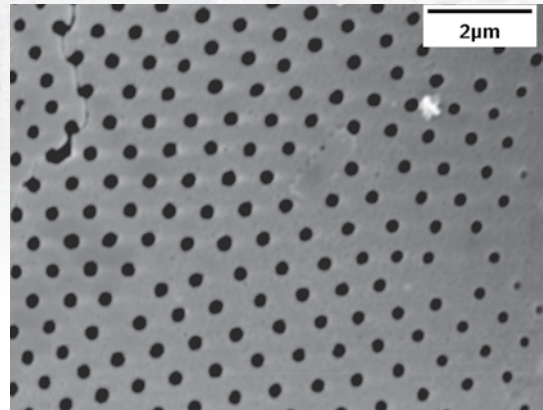
Figure 6. SEM photo of a portion of a centric diatom frustule exhibiting a lattice of pores. Magnification 11,000X. Scale bar = 2 microns.
