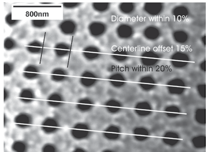
Figure 17. SEM photo of a portion of a centric diatom frustule exhibiting a lattice of circular pores. Magnification 34,000X. Scale bar = 800nm. Pore size = 250nm. Note that the diameters of these tiny pores are within 10% or 25nm of each other and the pitch (measurement from leading edge to leading edge) is within 20% or 63nm
