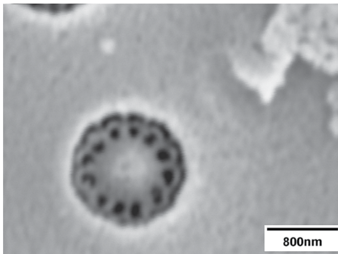
Figure 15. SEM photo of a portion of a triangular diatom frustule exhibiting ornamented pores. Magnification 30,000X. Scale bar = 800nm. Pore size = 88nm.
