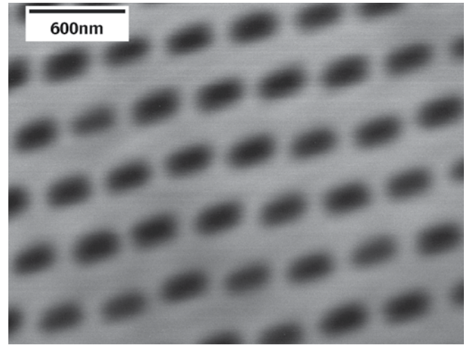
Figure 16. SEM photo of a portion of a centric diatom frustule exhibiting a lattice of oval pores. Magnification 40,000X. Scale bar = 600nm. Pore size = 200nm.
