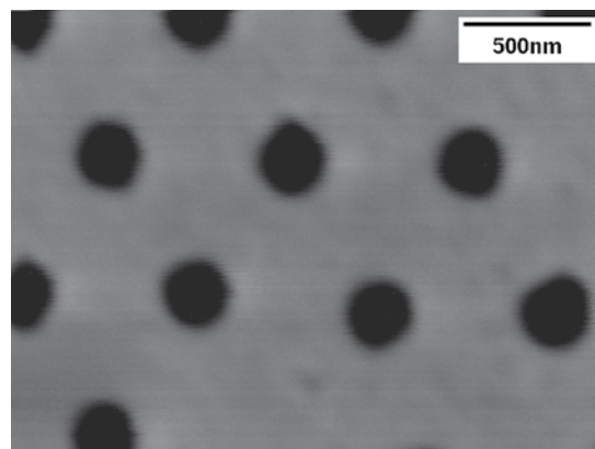
Figure 8. SEM photo of a portion of a centric diatom frustule exhibiting lattice of pores. Magnification 50,000X. Scale bar = 500nm. Pore size = 250nm.
