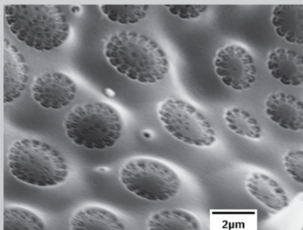
Figures 9–13. Various SEM photos of ornamented pores on triangular diatom frustules. Similar ornamentation on tiny pores is common.
