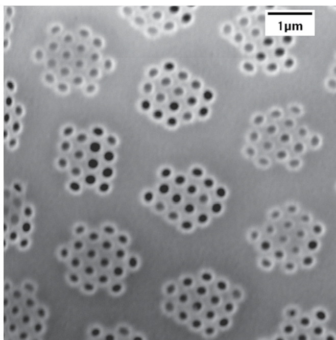
Figure 3. SEM photo of a portion of a centric diatom frustule exhibiting clusters of pores. Magnification 5,000X. Scale bar = 1 micron
