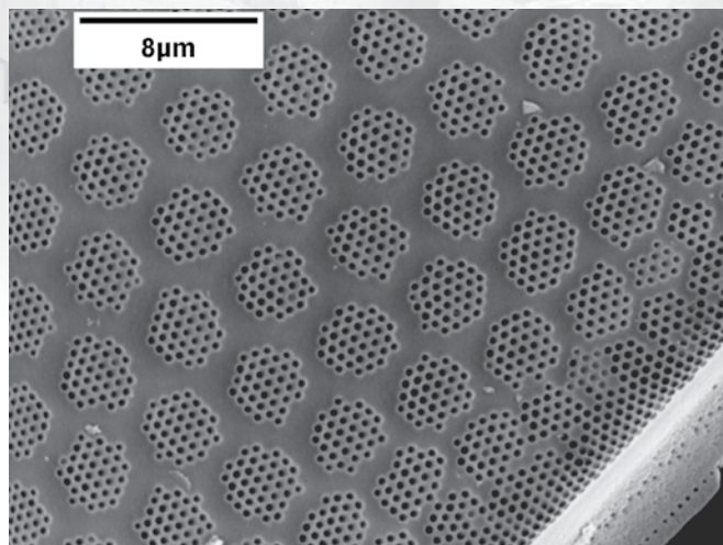
Figure 2. SEM photo of a portion of a centric diatom frustule exhibiting clusters of pores. Magnification 3,500X. Scale bar = 8 microns. A human hair is about 100 microns in diameter.
