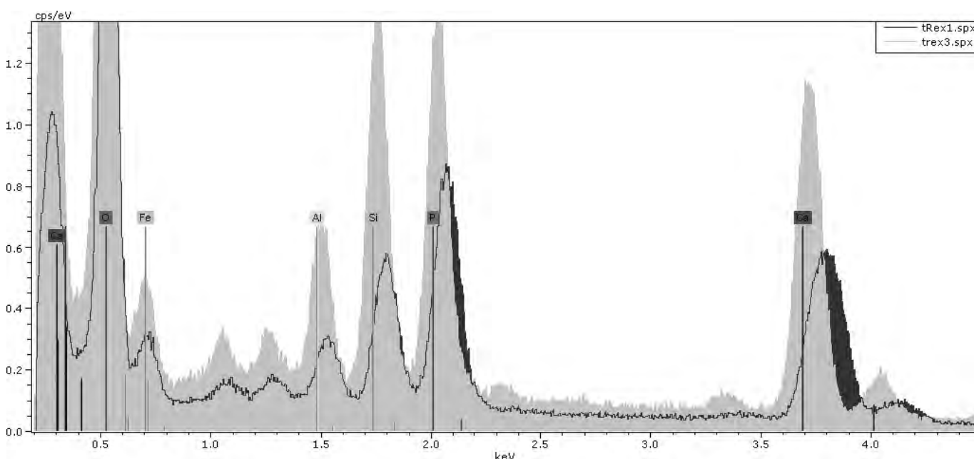
Figure 18. Composite of two of the three locations observed on the Tyrannosaurus rex right femur.
