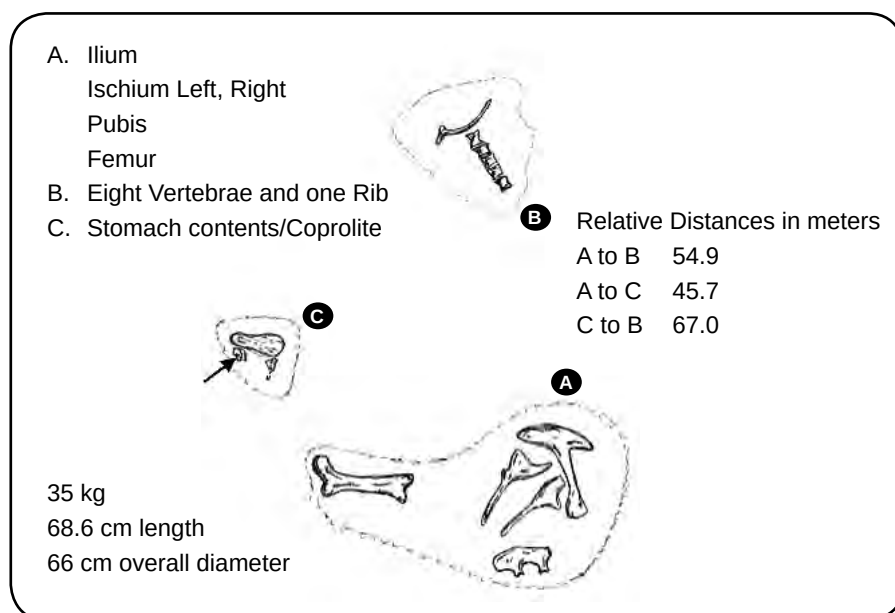
Figure 1. Map location of Tyrannosaurus rex excavation (August, 2009).
