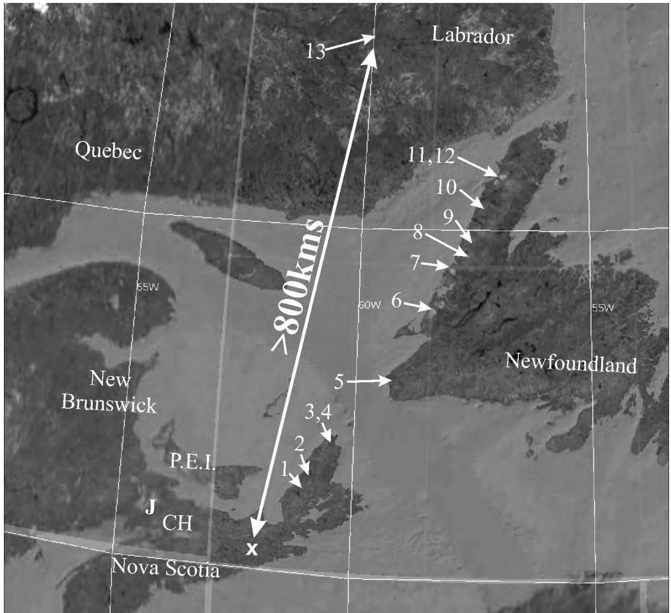
Figure 1. Map of significant points of interest along the Newfoundland Planation Surface.
