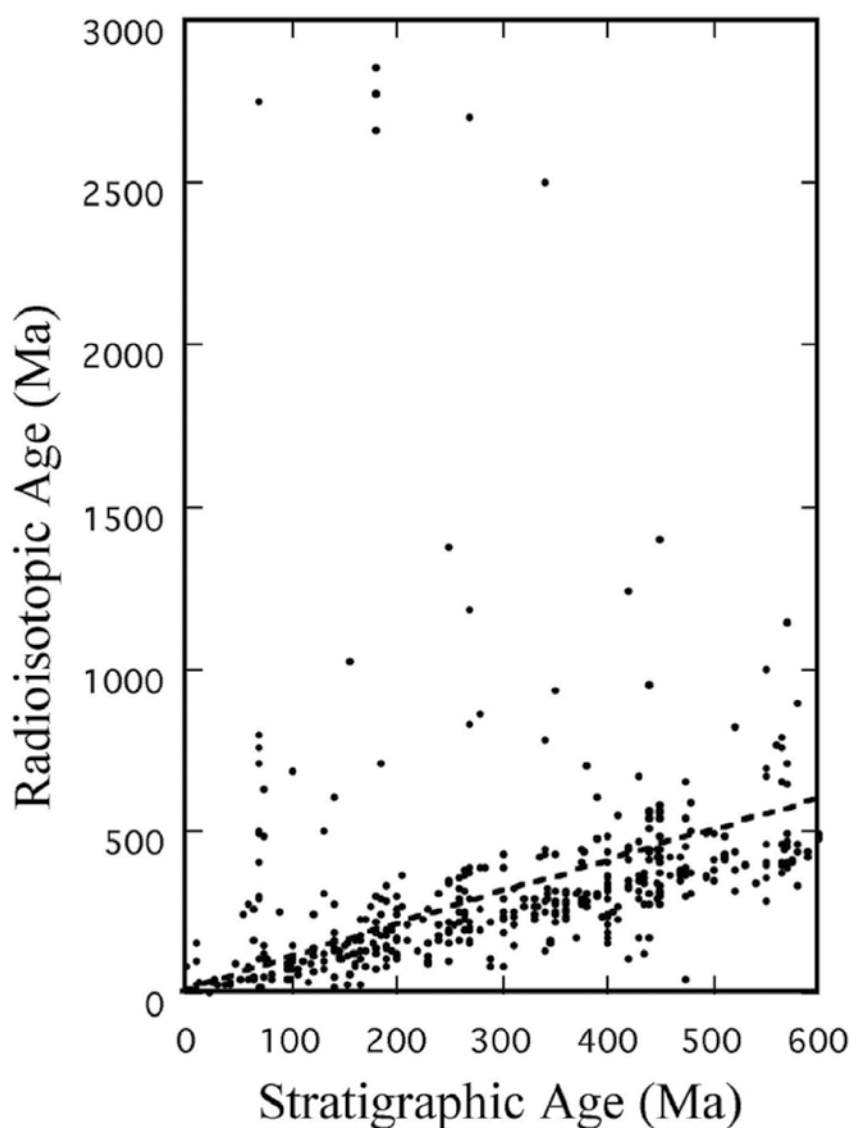
Figure 1. Published nuclear ages (not ^{14}\text{C} ages) compared to strata-determined geologic ages for the same rocks. Data picked for maximum deviation from the dashed line, where the data would lie if the two ages were always equal. Data also use a variety of methods (Woodmorappe, 1979).
