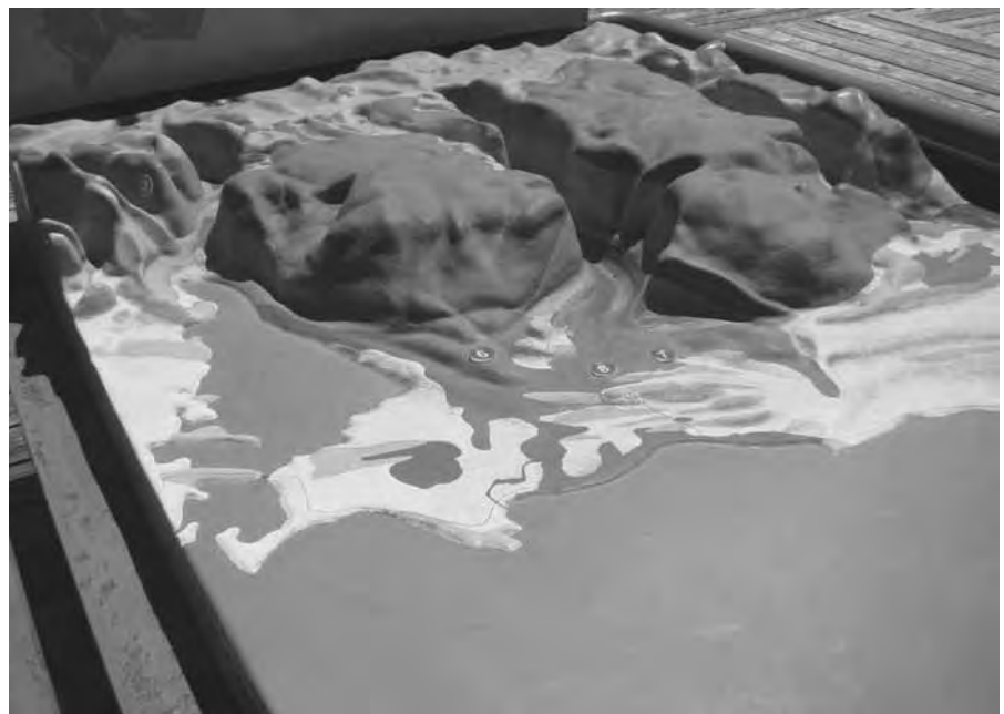
Figure 15. National Park model of the present-day Western Brook Pond area. Note the virtual absence of moraines and, even more importantly, the box-end that would best match the erosion of a waterfall cutting a canyon, rather than glaciers.
