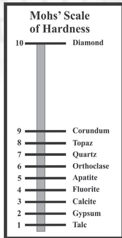
Figure 2. Geologists have created a subjective scale of hardness (Mohs' scale of hardness). The numbers are relative and only indicate that one mineral is harder or softer than the one adjacent to it. The ten minerals identified are the standard, and everything else is applied in relation to those standards. Diamond is significantly harder than the minerals below it, and its distant location up the scale is reflective of that difference. Zircon has been identified as having a hardness of 7.5. This does not mean that it is 7.5 times harder than talc (hardness of 1); rather, it is harder than quartz (7.0) and softer than topaz (8.0). We suggest great caution when assuming that minerals on this scale above a certain value are believed by their hardness to reflect impenetrability.
