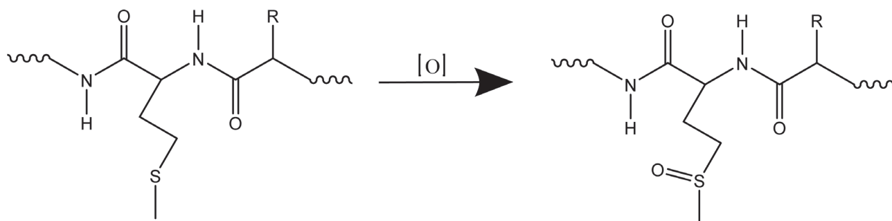
Figure 5. Oxidation of methionine residue to methionine sulfoxide.
