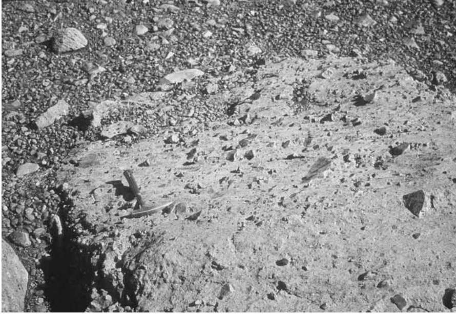
Figure 8. Breccia boulder deposited by Skeiðarárjökull, photographed in 2002.
