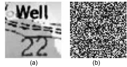
Figure 1. 50 x 50-pixel image of a small section of a topographic map. The correctly digitized (scanned) image is shown in (a), while the scrambled pixels shown in (b) represent one redistribution of the 2500! ( 1.63 \times 10^{7,411} ) possible permutations of the pixels for this image. 50 x 50 pixels is roughly 1/6^{\text{th}} of the foveal FOV for human eyes.
