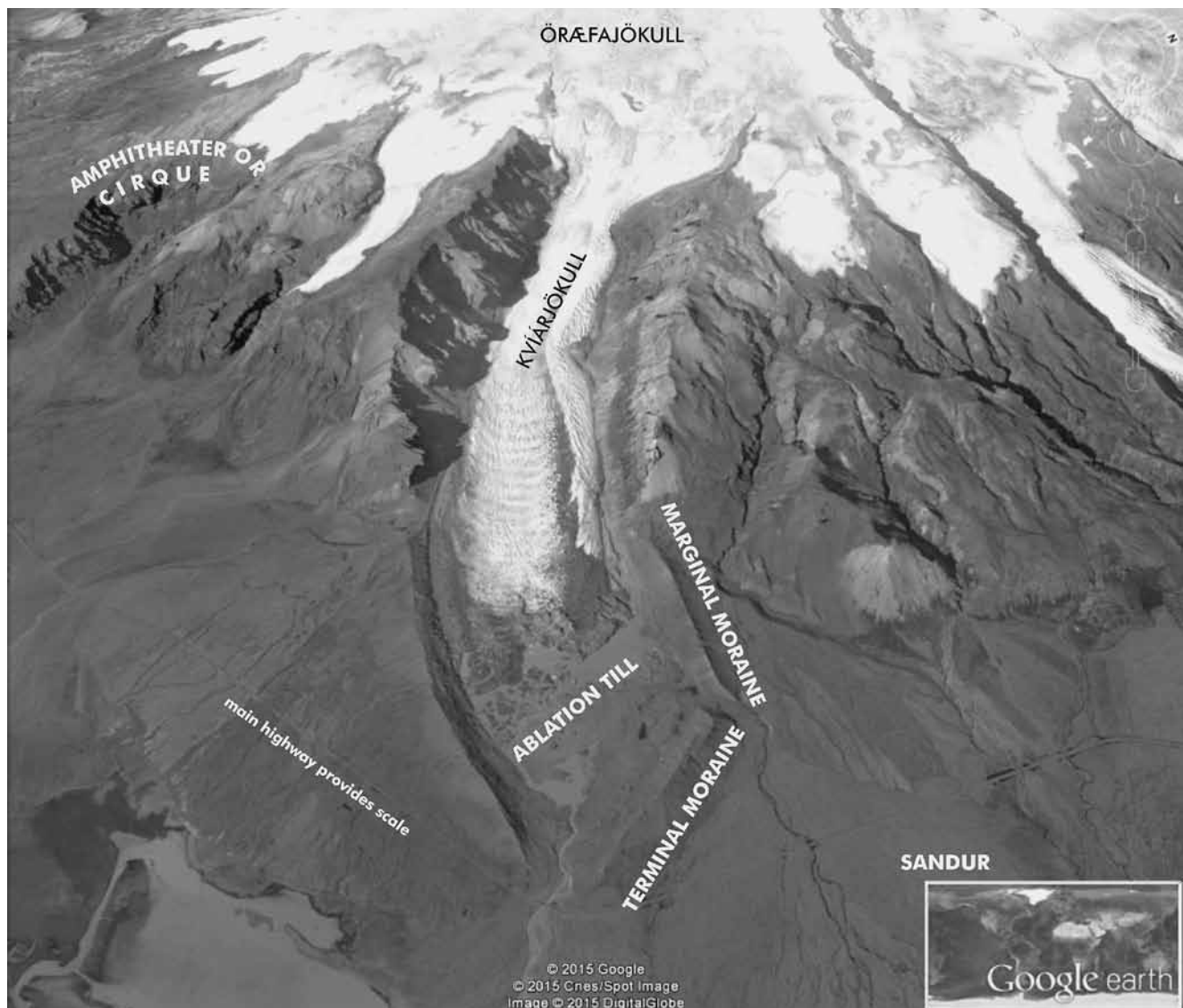
Figure A4. Öräfajökull is the ice cap on Öräfi, the high mountain at the south end of Vatnajökull. Kvíárjökull is the most prominent outlet glacier from Öräfajökull and occupies a deeply cut valley. The terminal moraine arrested the advance of the glacier during the Little Ice Age (Ives, 2007). The other outlet glaciers tend to move less ice and produce less erosion as a result. The prominent erosional feature to the left (northwest) may be an amphitheater produced by mass wasting, a cirque eroded by a glacier, or as seems likely, an amphitheater in which ice contributed to enlargement during the Little Ice Age. Oblique Google Earth view.
