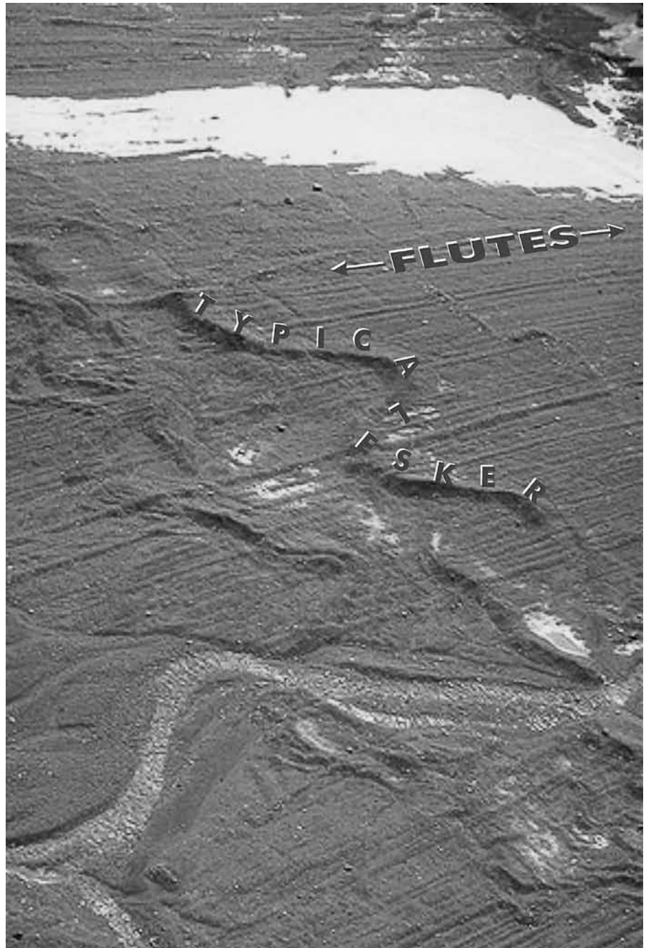
Figure 22. Flutes and eskers indicated on aerial base image of Bear Glacier, Kenai Peninsula, Alaska. This forefield lies behind the Little Ice Age terminal moraine. Base image from Eastern Illinois University ( http://www.ux1.eiu.edu/~cfjps/1300/glacier_photos.html ).
