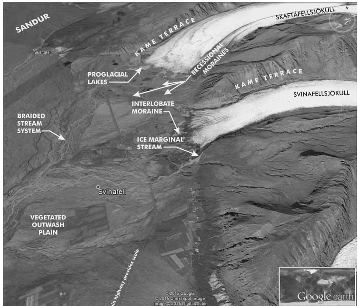
Figure A3 ( below ). A closer view of the area shown in Figure A2, showing various glacial landforms produced by Skaftafelljökull and Svinafelljökull, mostly during the Little Ice Age.
