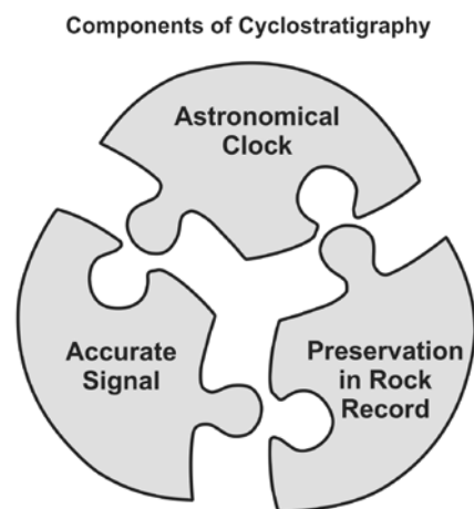
Figure 4. Cyclostratigraphy depends on the reality and accuracy of an astronomical clock, the accurate relay of the time signal to Earth via astronomically forced climate variation, and the preservation of these variations in sedimentary units that both capture this signal and are sufficiently sensitive to record its small changes in chemical, biogenic, and sedimentary fluctuations.
