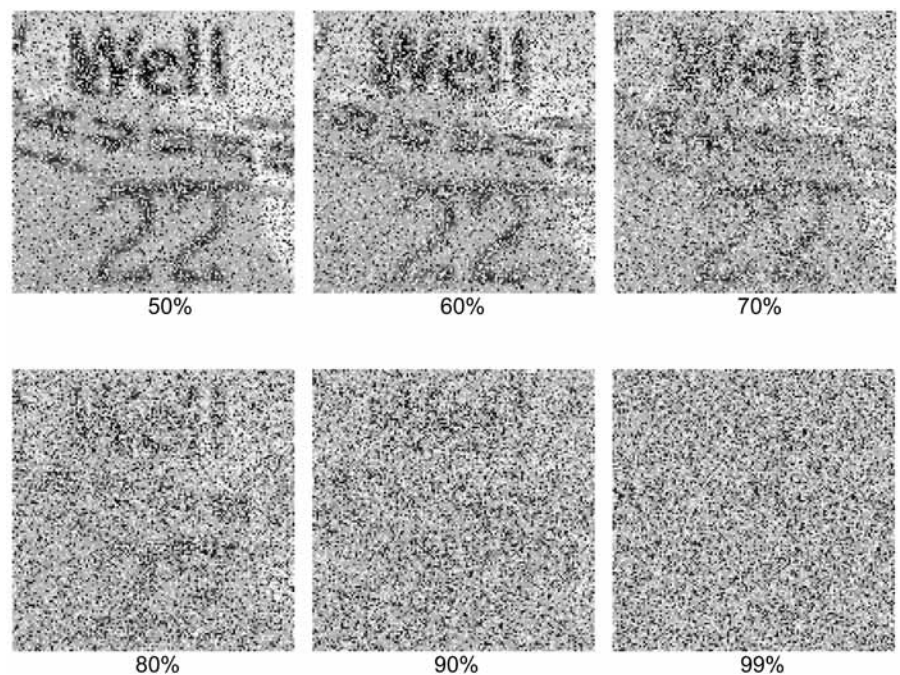
Figure 2. The pixels of Fig 1(a) have been randomized at various levels, indicated by the percentages.
