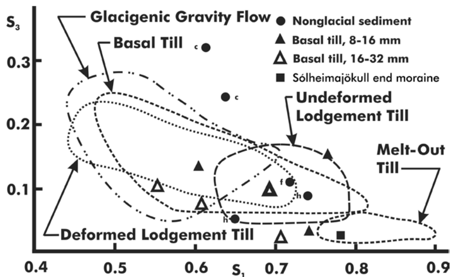
Figure 9. Fabrics in unconsolidated sediments can be useful indicators of probable origin, but they are not diagnostic. Fabric strength envelopes from Dowdeswell and Sharp (1986). These were derived primarily from Breiðamerkurjökull (See Figure 2 for locations). Nonglacial fabrics (•) from Klevberg and Oard (2005): c—colluvium, f—fluvial floodplain gravel, h—hypothetical (computer-generated fluvial). Also shown are basal till fabric data from 1980 surge of Vestari-Hagafellsjökull (Carr and Goddard, 2007) for 8–16 mm fraction (▲) and 16–32 mm (△), and end moraine fabric from Brynjólfsson (2004) left after the advance of Sólheimajökull that ended in 1995 (■).
