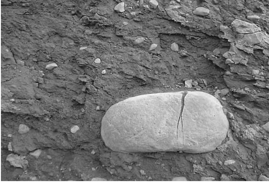
Figure 6. Lodgement till in drumlin, Sólheimajökull forefield, photographed in 2004 (from Ingólfsson, 2008).
