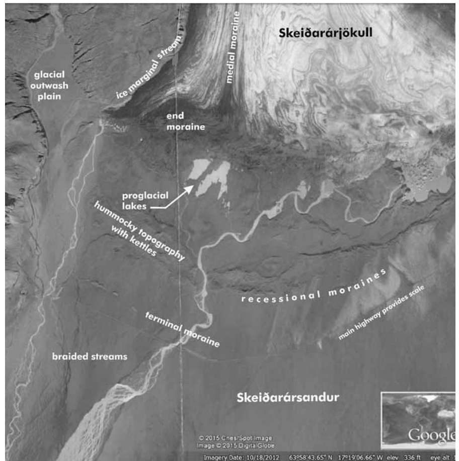
Figure A1. Aerial photomosaic of snout of Skeiðarárjökull with glacial landforms labeled. Meltwater channels have shifted frequently through the years.
