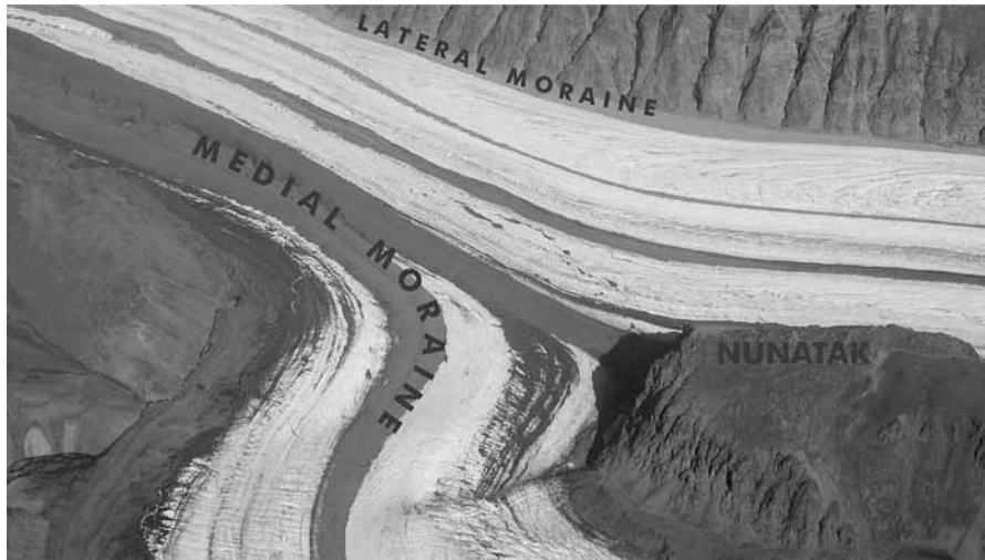
Figure 15. Moraines and Nunatak on Nuussuaq Peninsula, Greenland. Base image from Wikipedia Commons.
