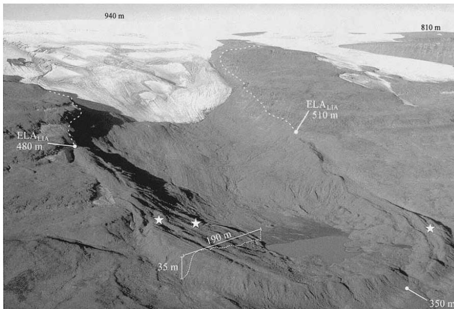
Figure 16. Moraines from Little Ice Age with equilibrium line altitude (ELA) contemporary with moraine formation indicated. Rock glacier on southwest Diskø, Greenland (Figure 1). Star symbols represent sampling locations. Figure from Humlum (2000).
